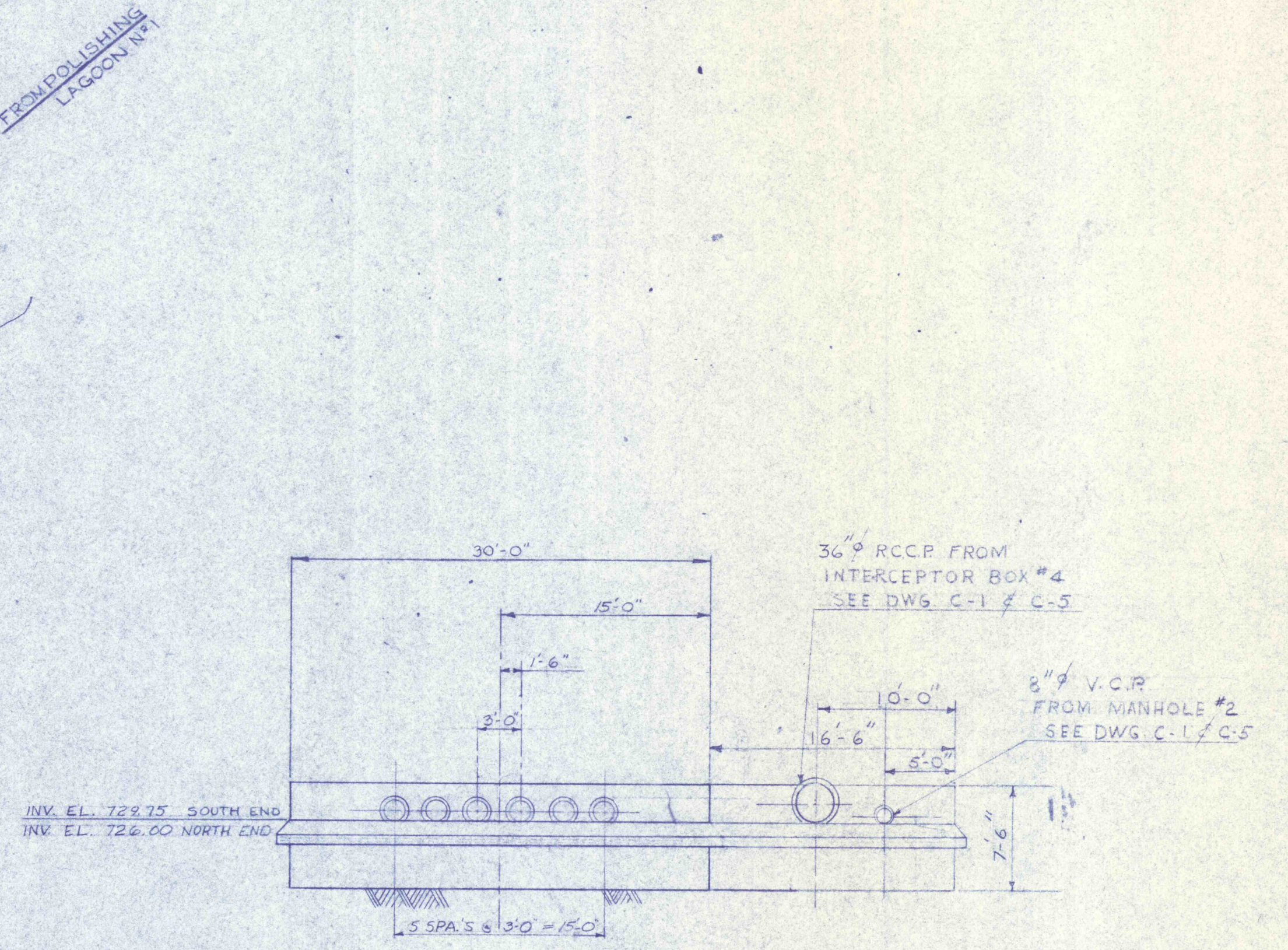
SECTION B-B
