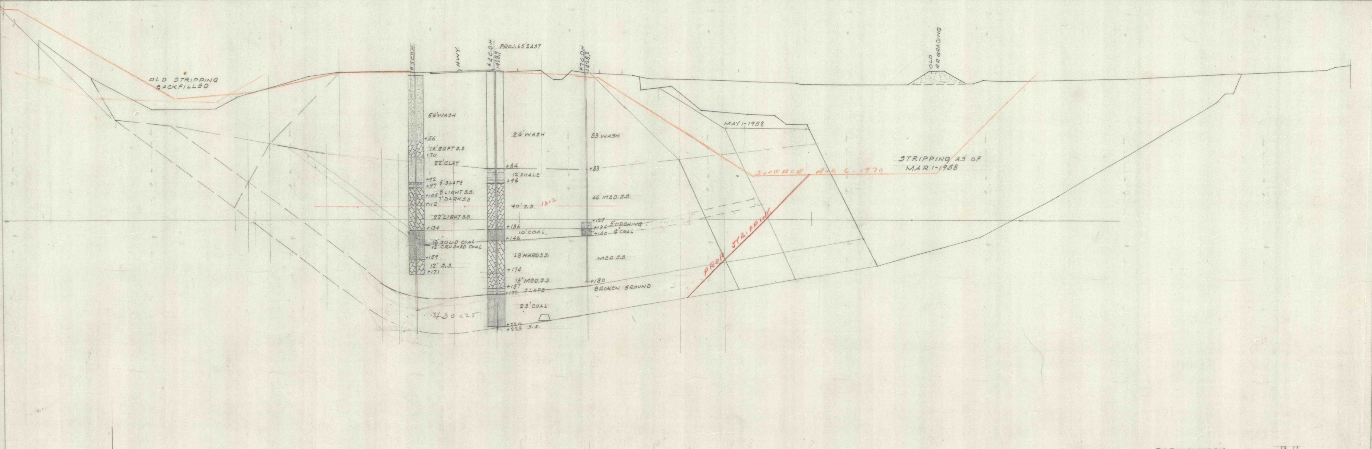
LOGAN STRIPPING SECTION 58+00 EAST SCALE 1"=50' 4-16-58
