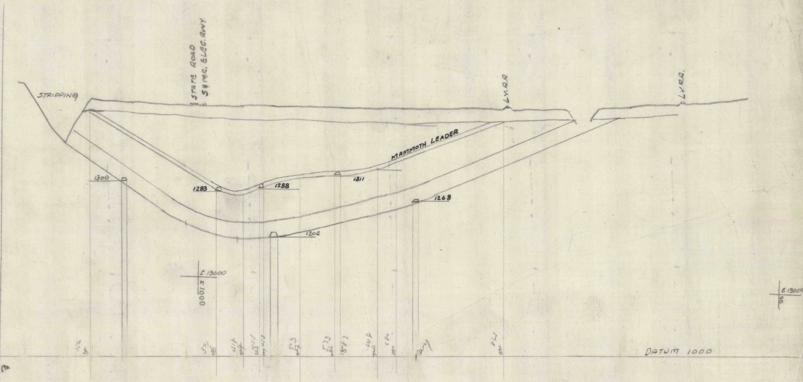
SECTION No 6
