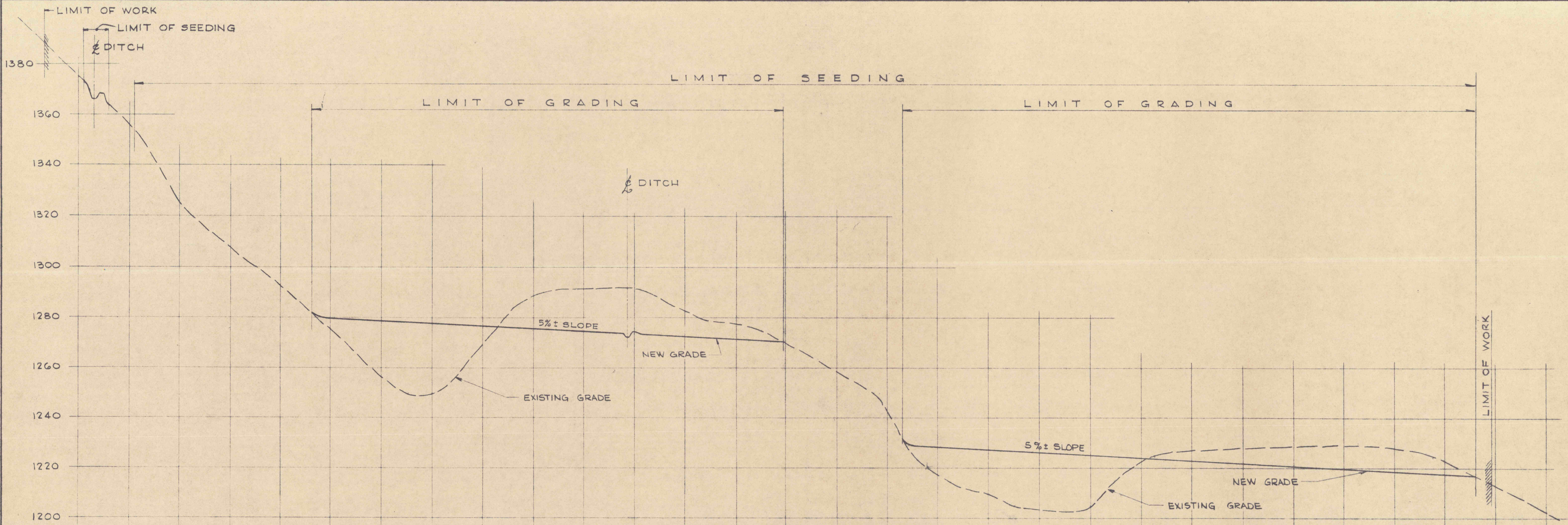
CROSS-SECTION NO. 3 SCALE: 1" = 20' (HORIZ. & VERT.) FOR LOCATION SEE DRAWING NO. 2
