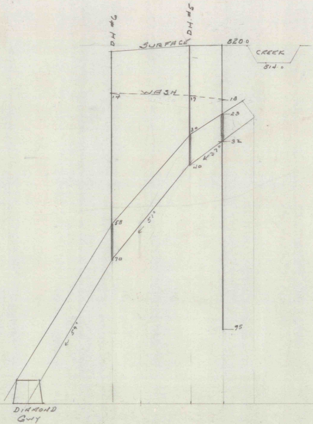
FORESTVILLE SECTION SHOWING DRILLING TO FIND OPENING IN MINE WORKINGS SCALE 1"=20'
