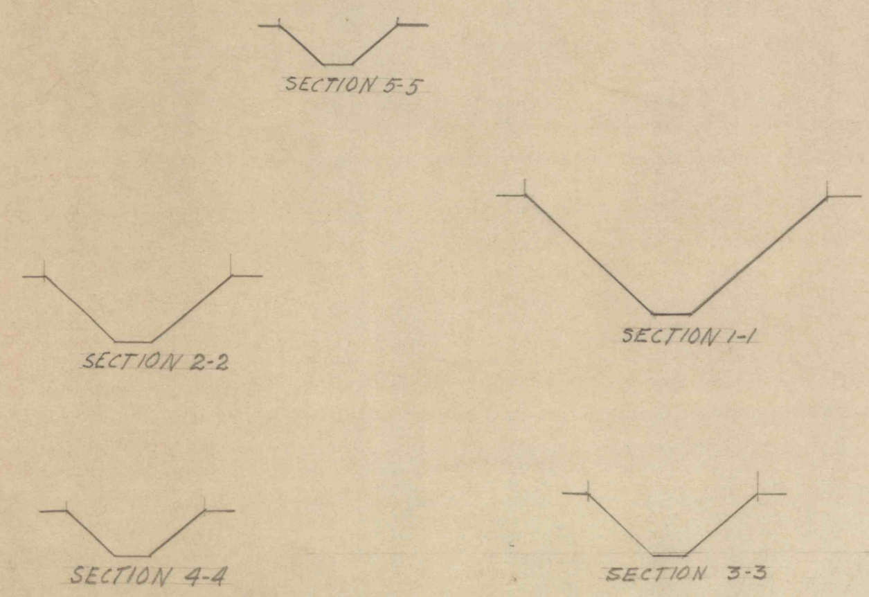
SECTIONS OF PIPE TRENCHES
