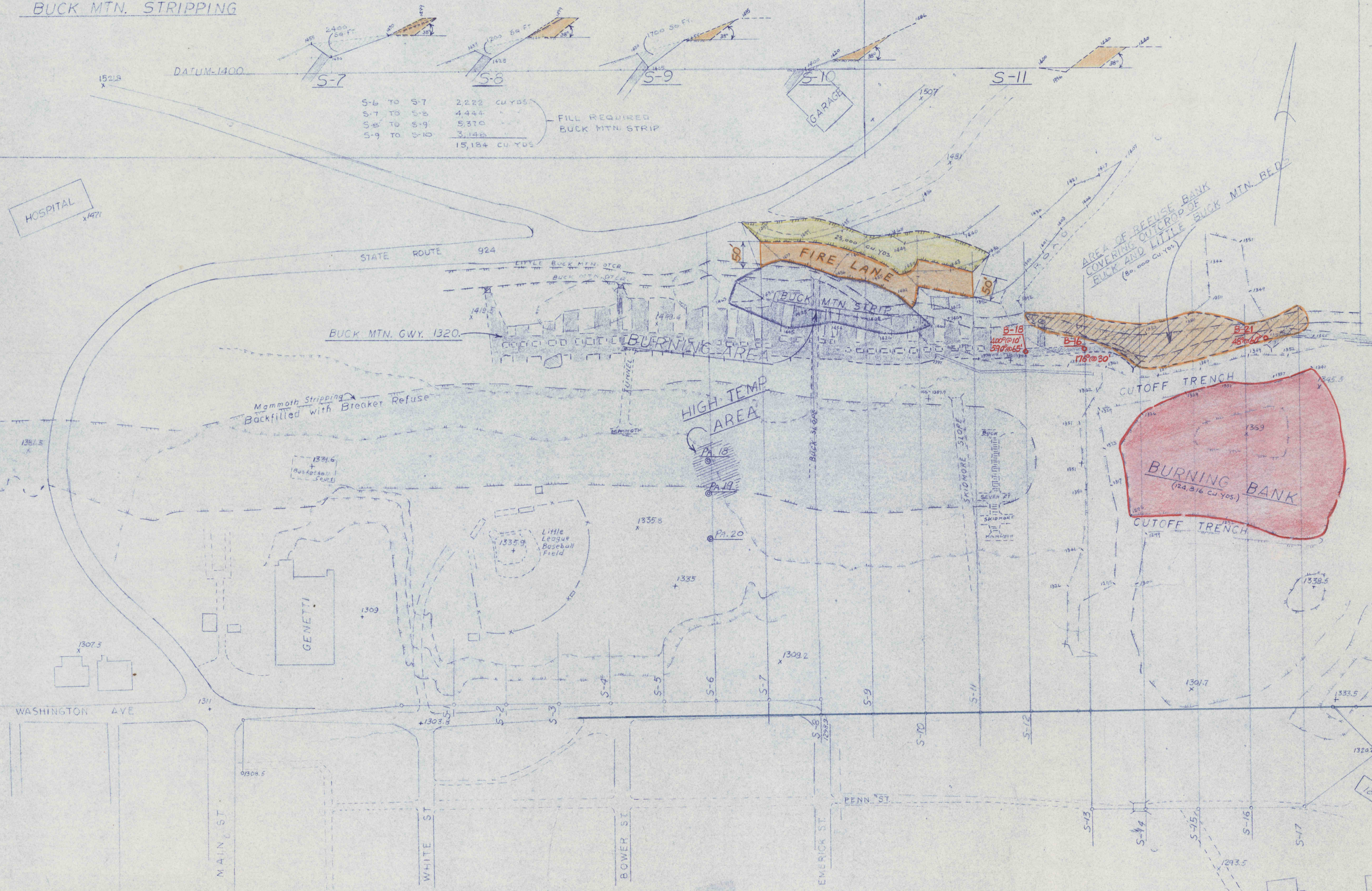
KEHLEY RUN MINE FIRE STRIP PIT BACKFILL - BANK REMOVAL Scale 1" = 100'
