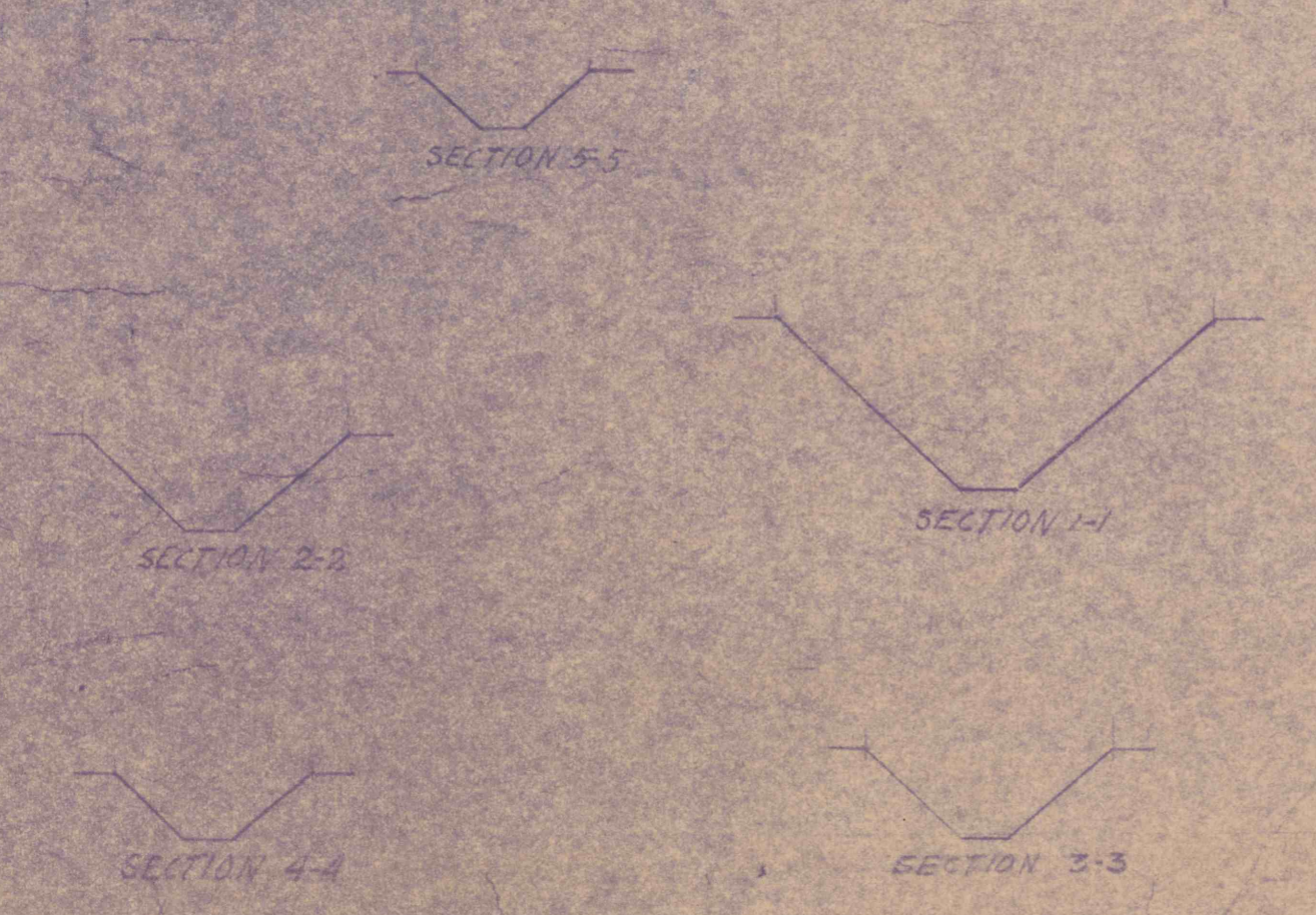
SECTIONS OF PIPE TRENCHES
