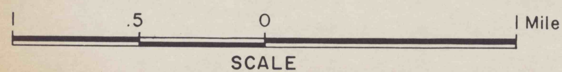
FIGURE 23 CARBONDALE QUADRANGLE
