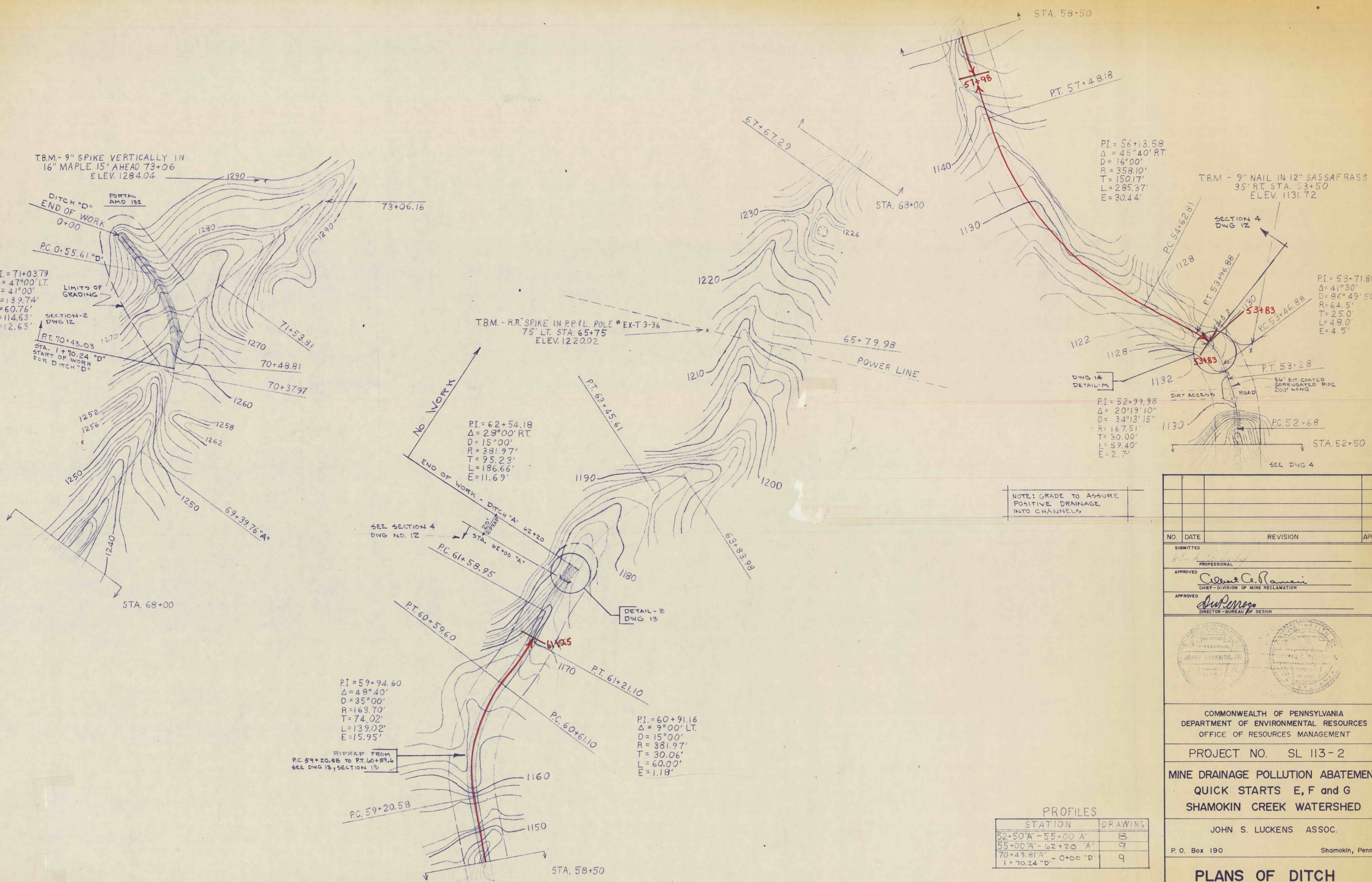
PLANS OF DITCH "A" & "D" SCALE - 1" = 50' - 0"
