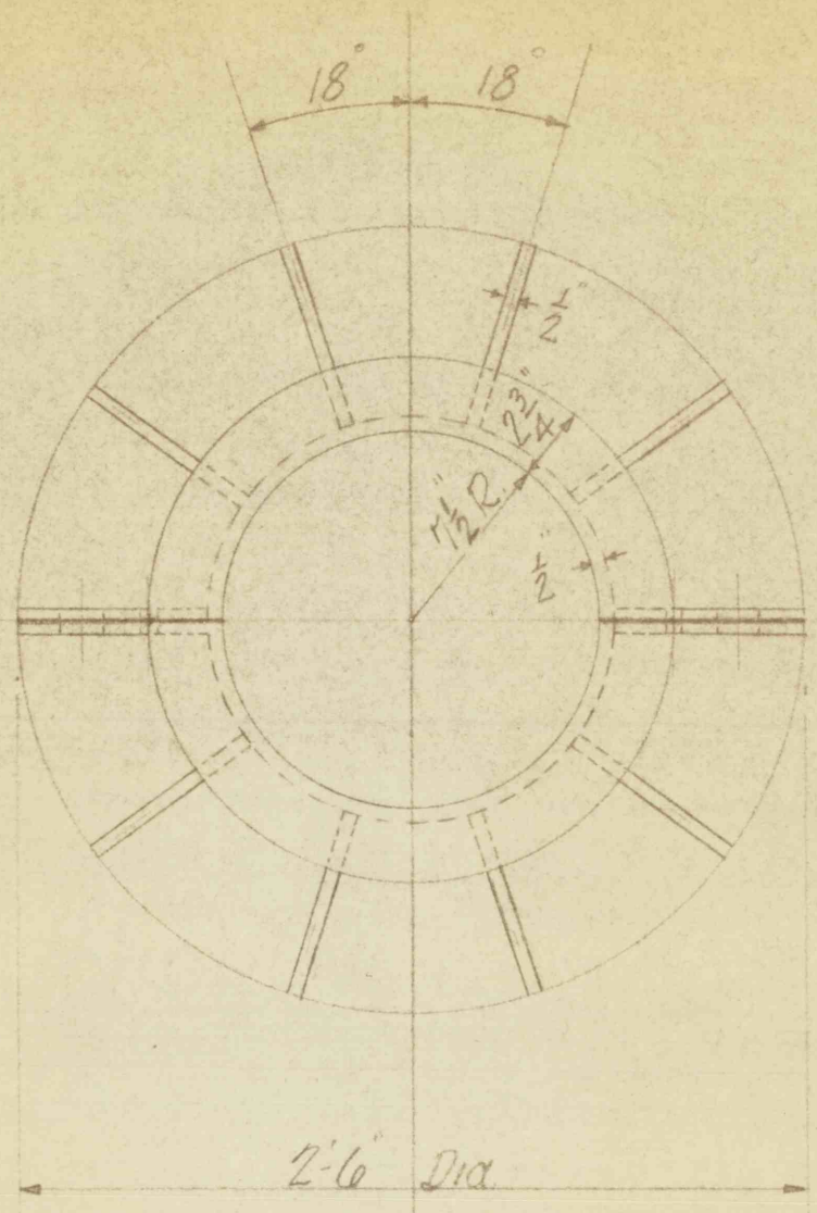
PLAN
