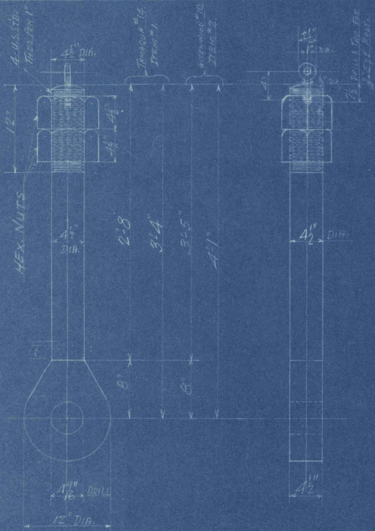
4 1/2" DIA. SPECIAL EYE BOLT. ITEMS #1 & #2.
