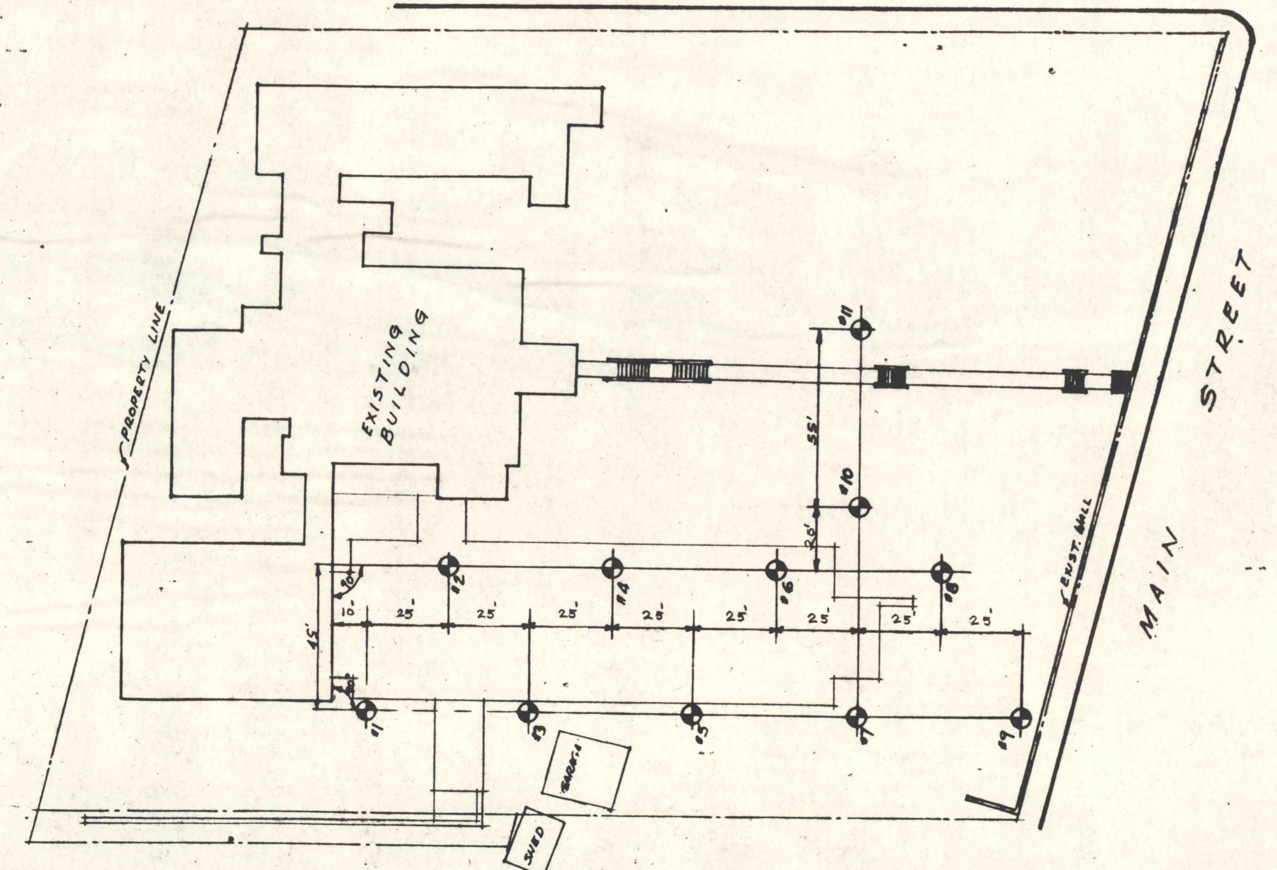
TEST BORING PLAN SCALE 1"=30.0'
