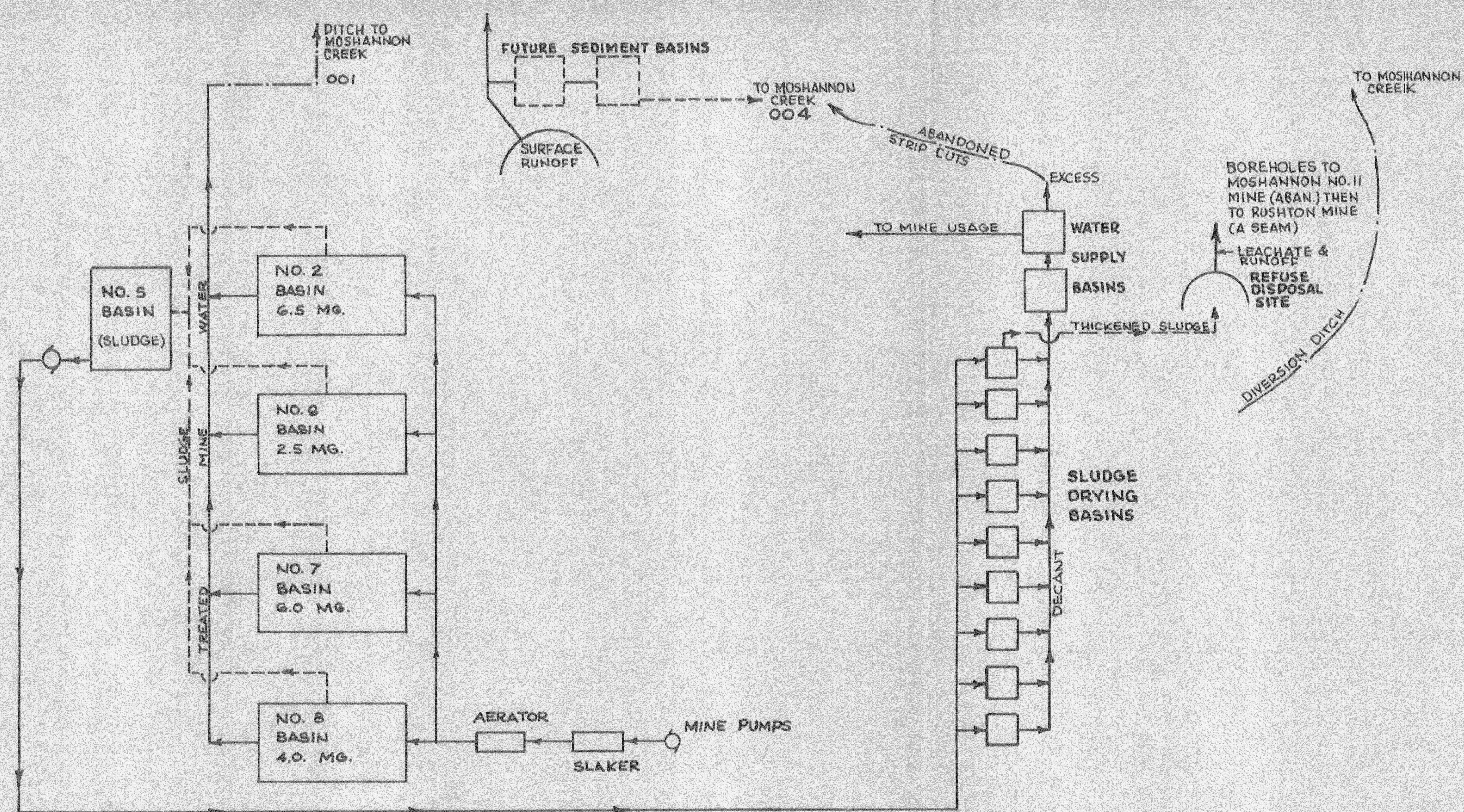
SCHEMATIC FLOW DIAGRAM PROPOSED NEW SYSTEM
