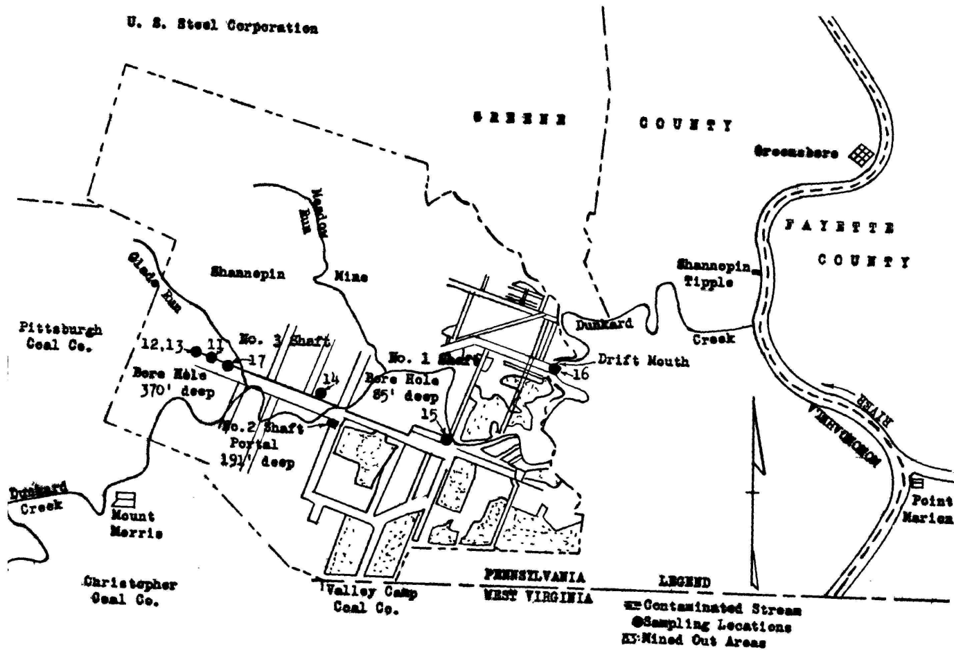
Figure 4. - Sketch map of Pittsburgh bed and surface at the Shannopin mine of Jones and Laughlin Steel Corporation.
