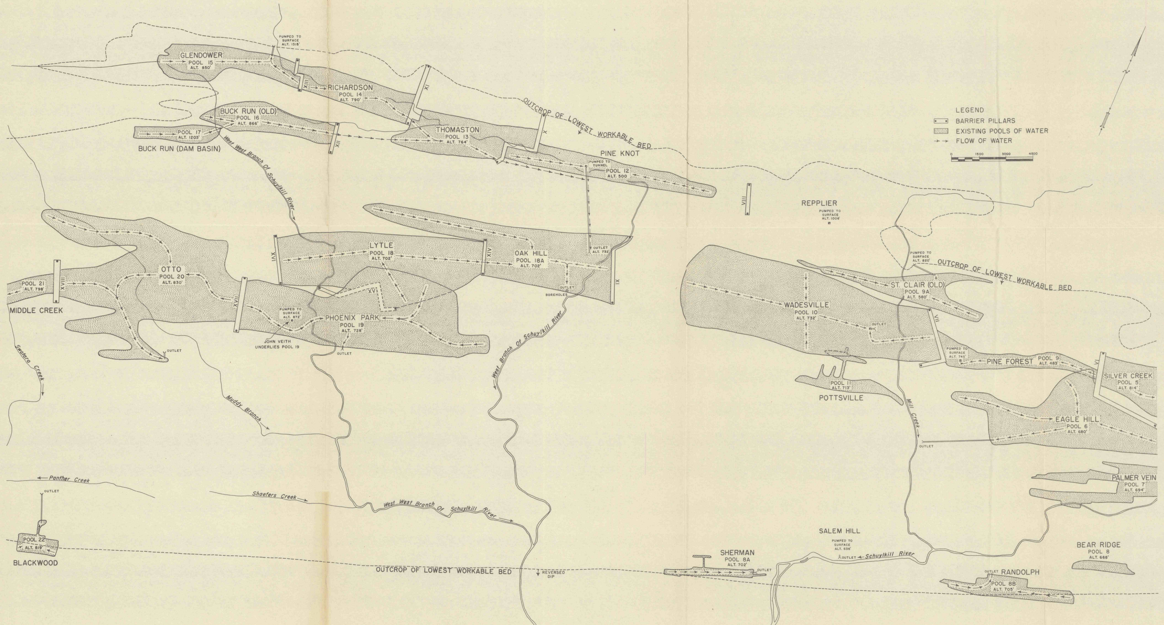
FIGURE 24.—Map Showing Direction and Path of Flow of Mine Water Into and Out of Mines Affected by Barrier-Pillar System in Central Part of Area Studied in Southern Field.
