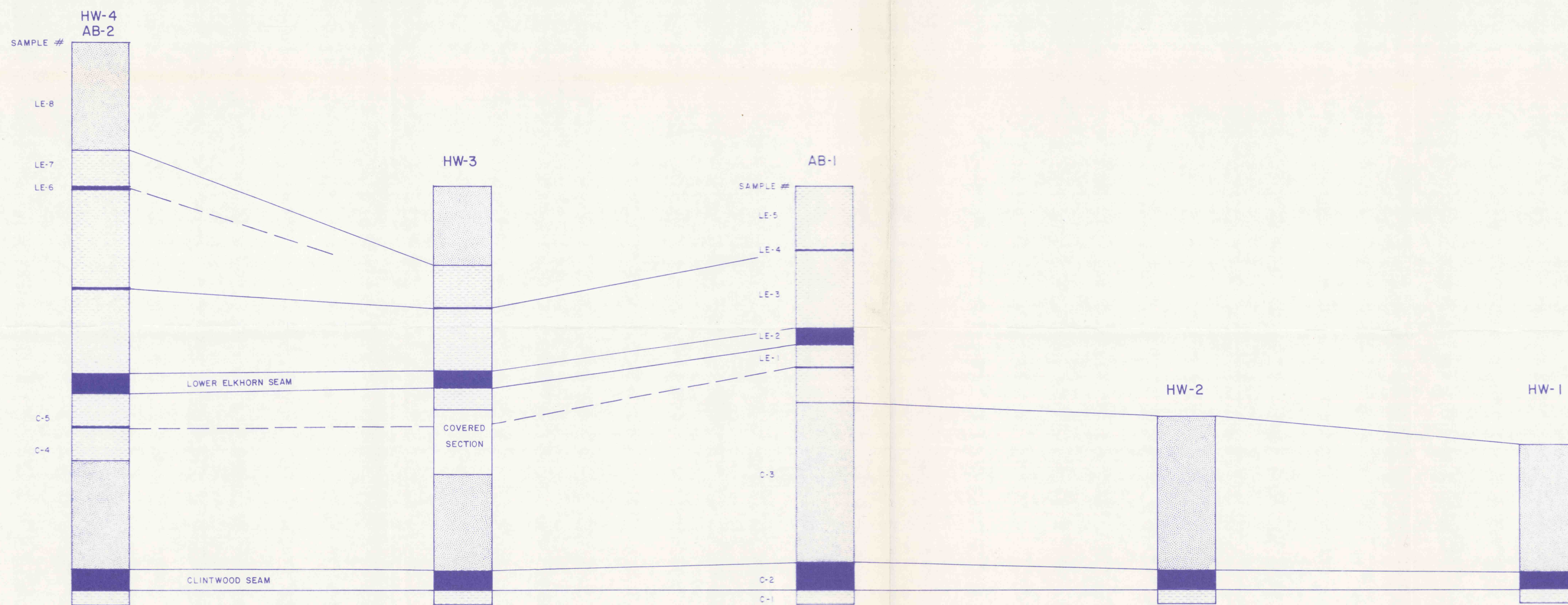
SECTION A-CLINTWOOD AND LOWER ELKHORN SEAMS
