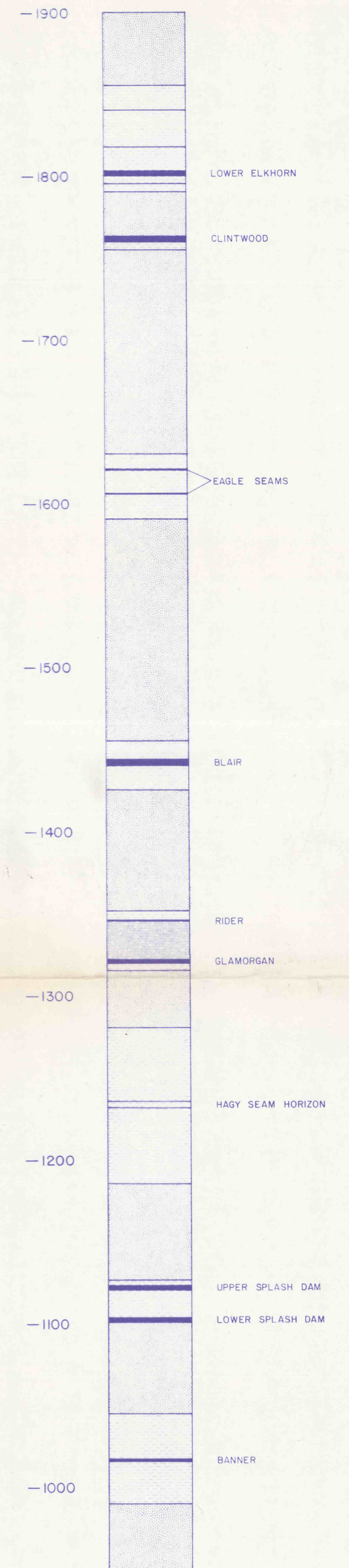
GENERALIZED STRATIGRAPHIC COLUMN SCALE 1" = 50'
