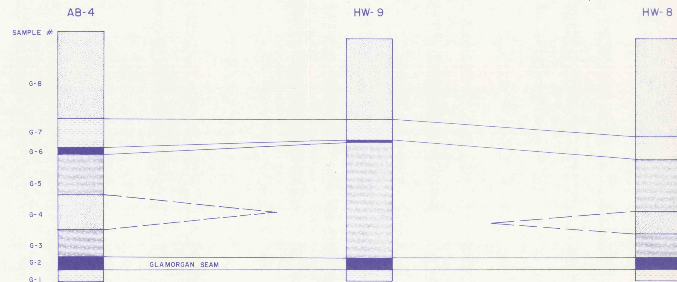
SECTION C-GLAMORGAN SEAM
