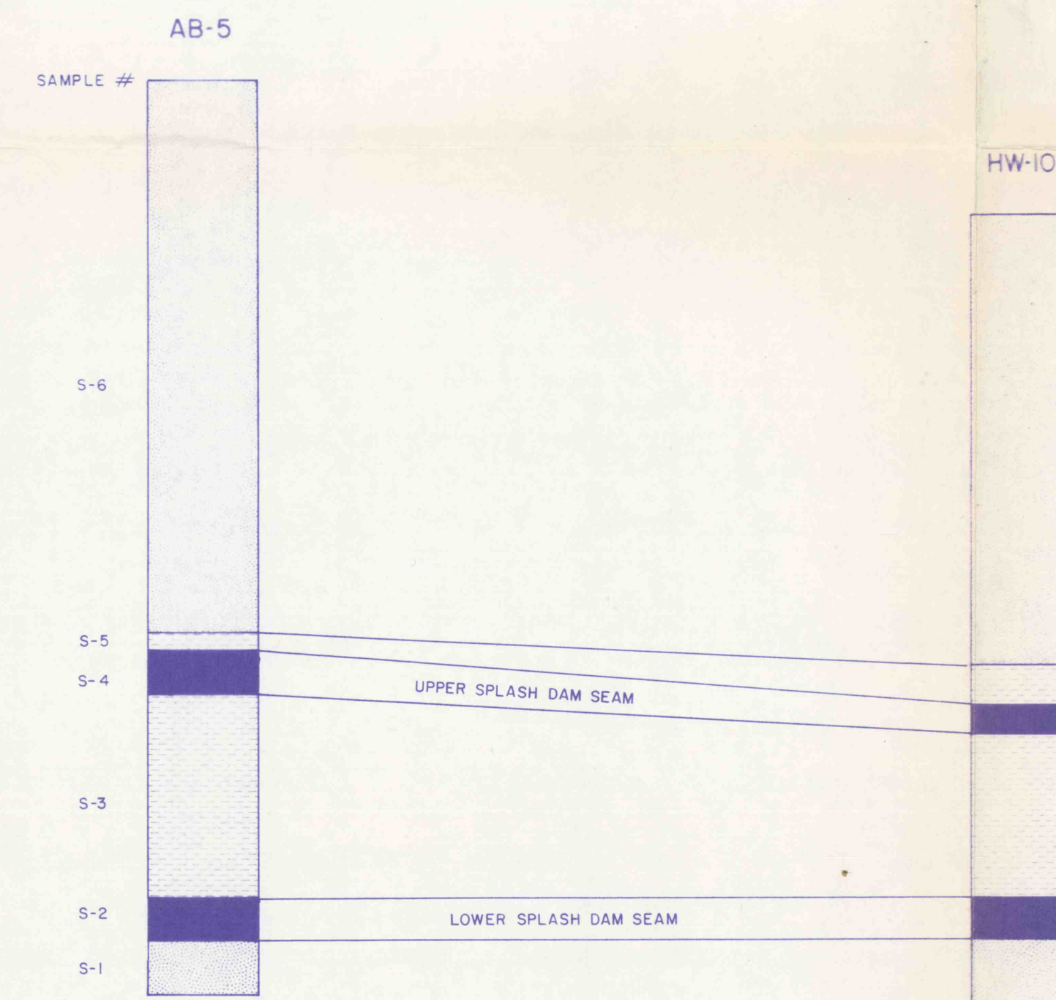
SECTION D-UPPER AND LOWER SPLASH DAM SEAMS
