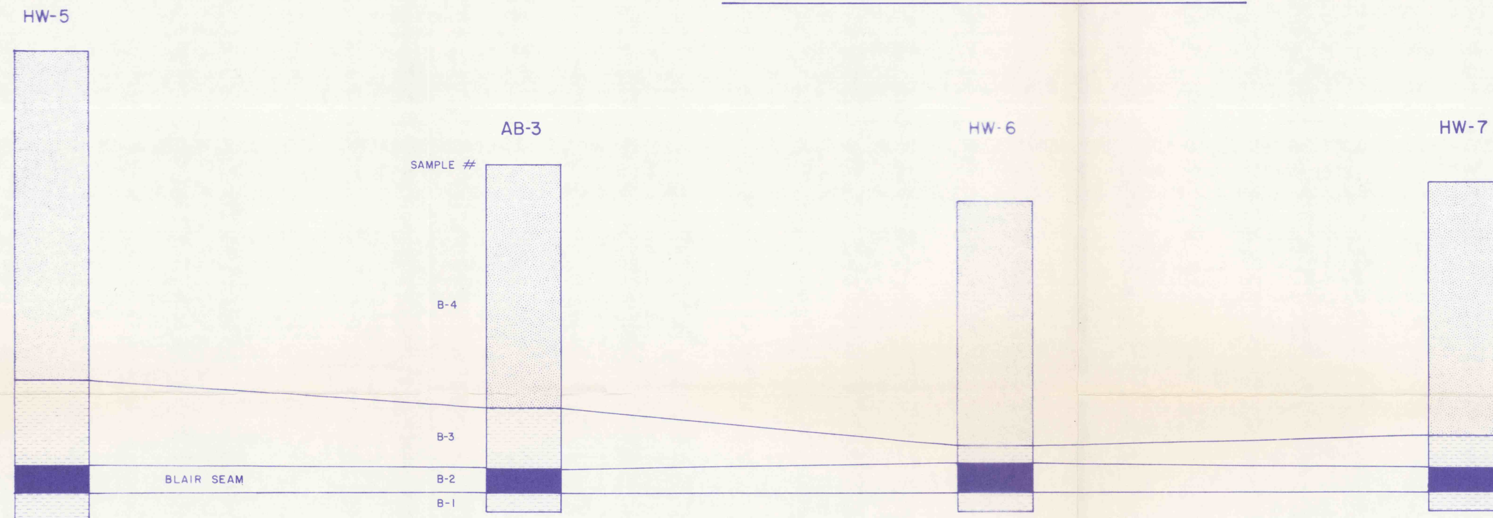
SECTION B-BLAIR SEAM
