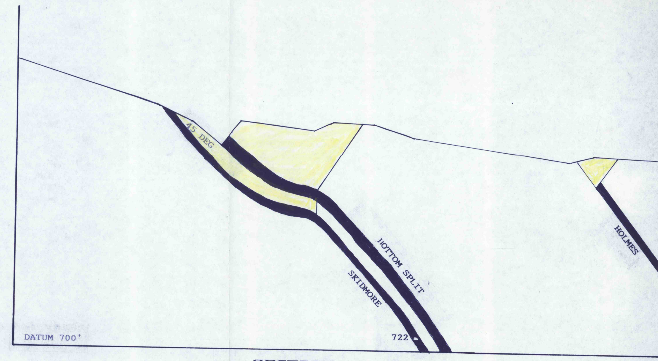
SECTION L - L
