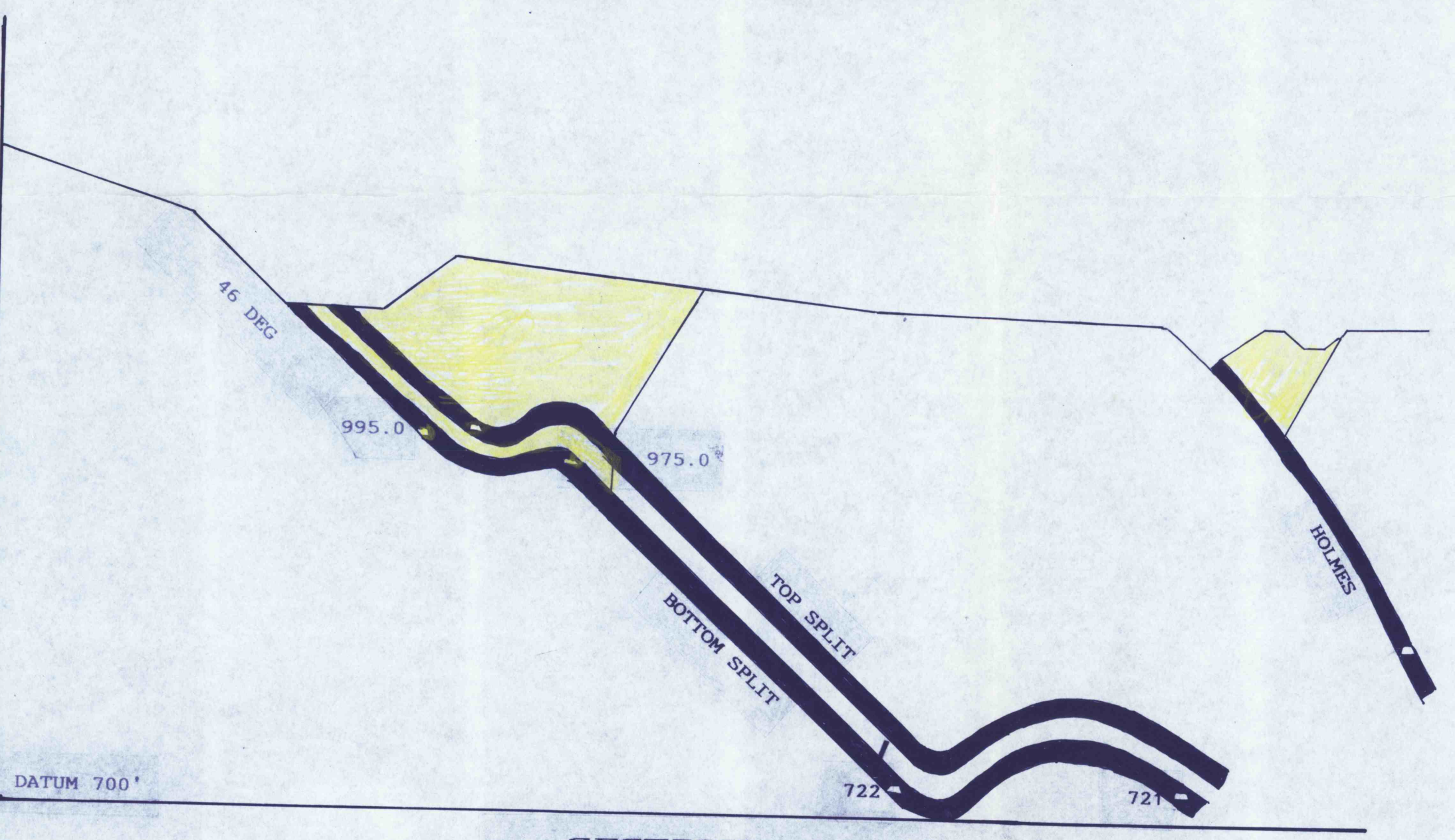
SECTION J - J
