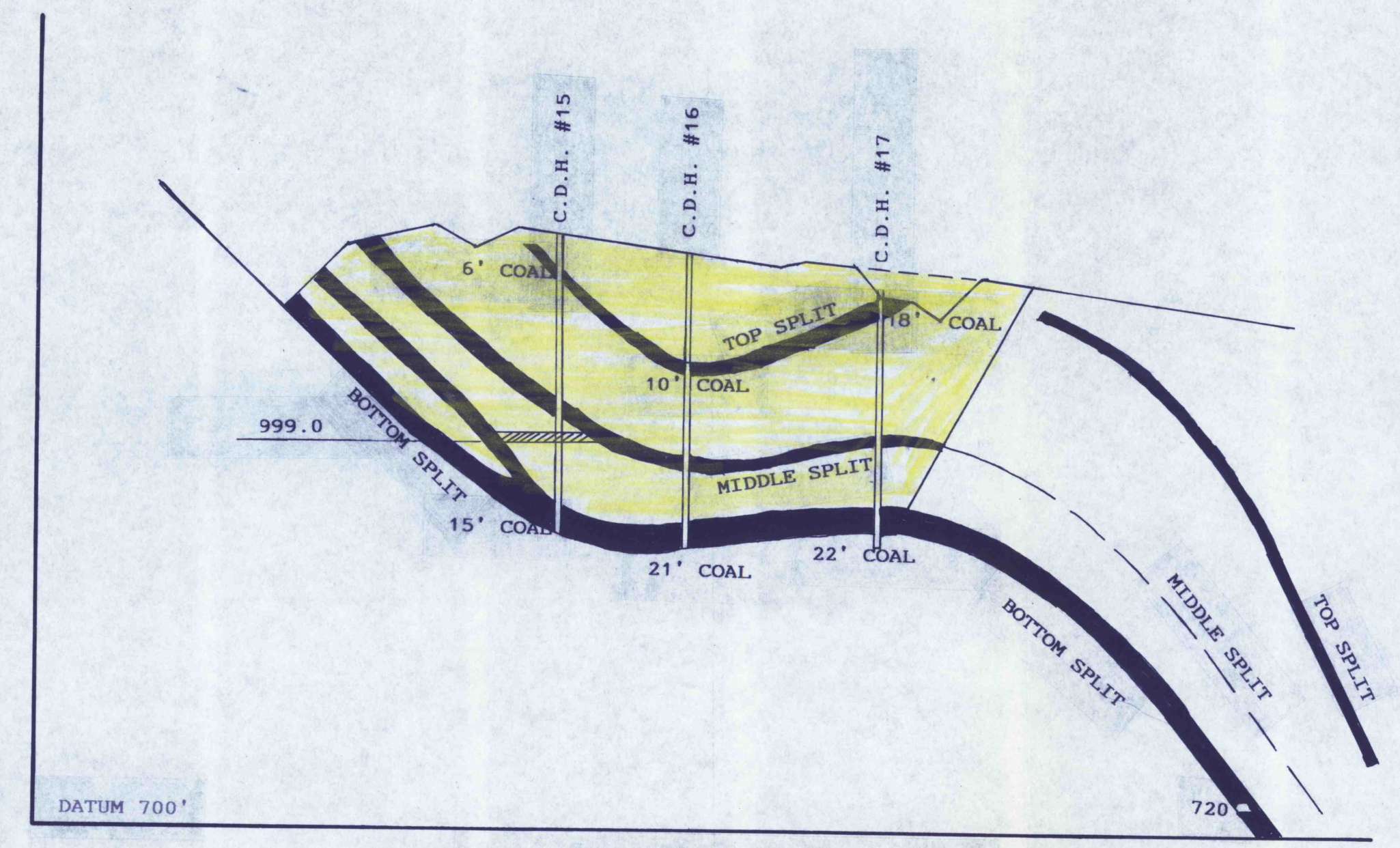
SECTION H - H
