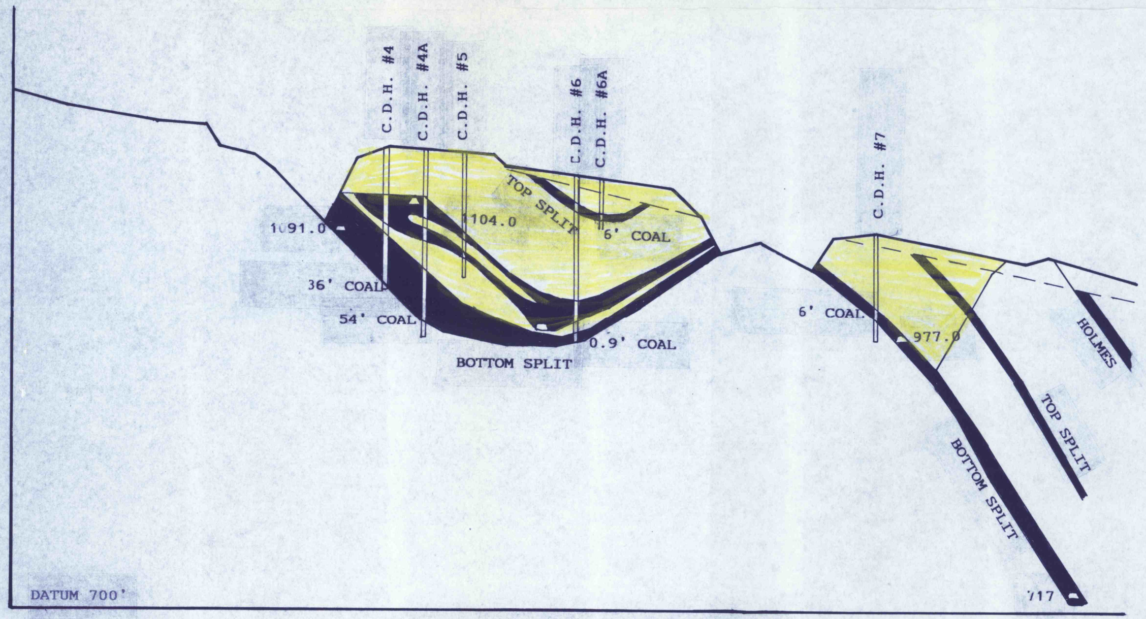
SECTION F - F
