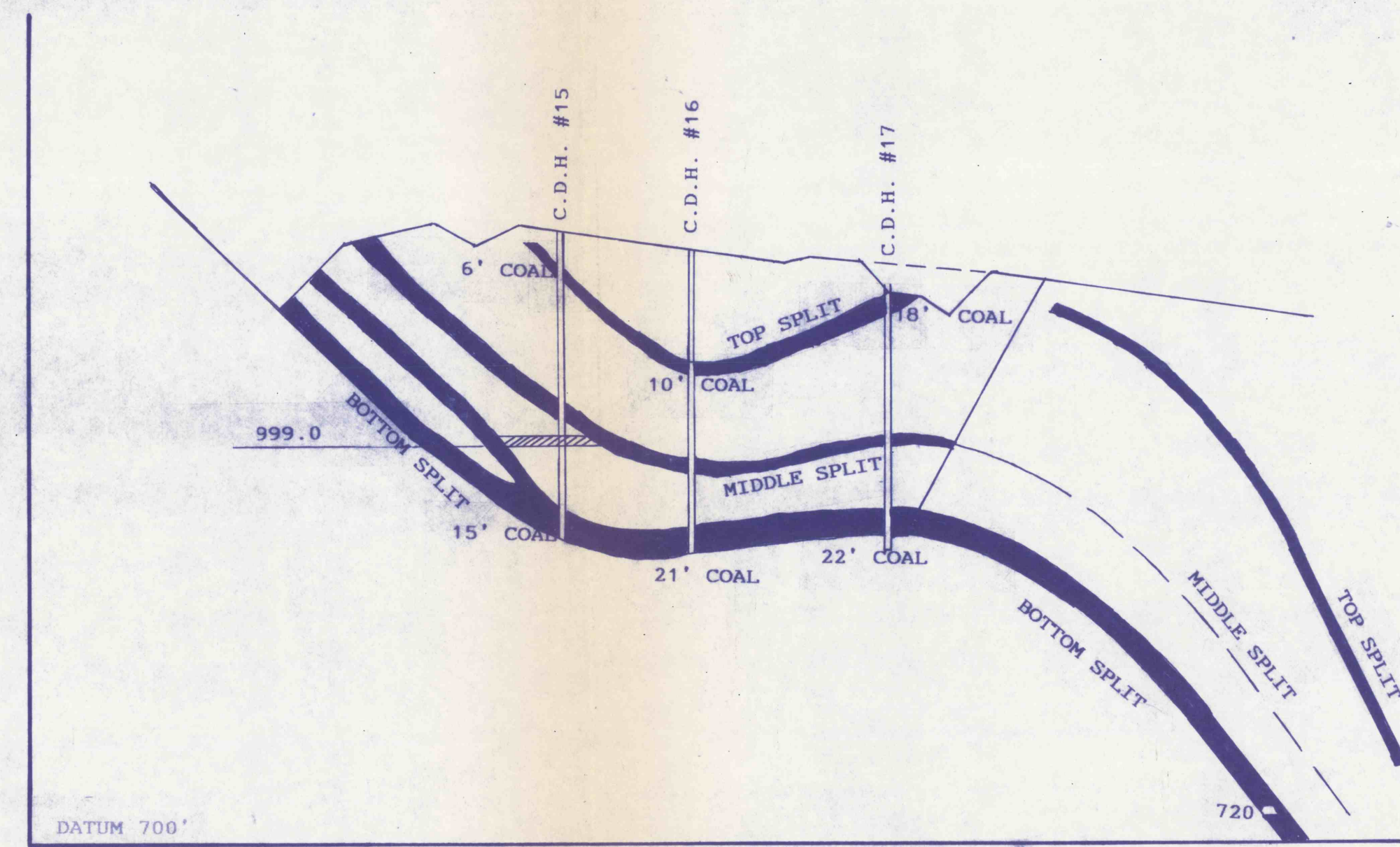
SECTION G - G
