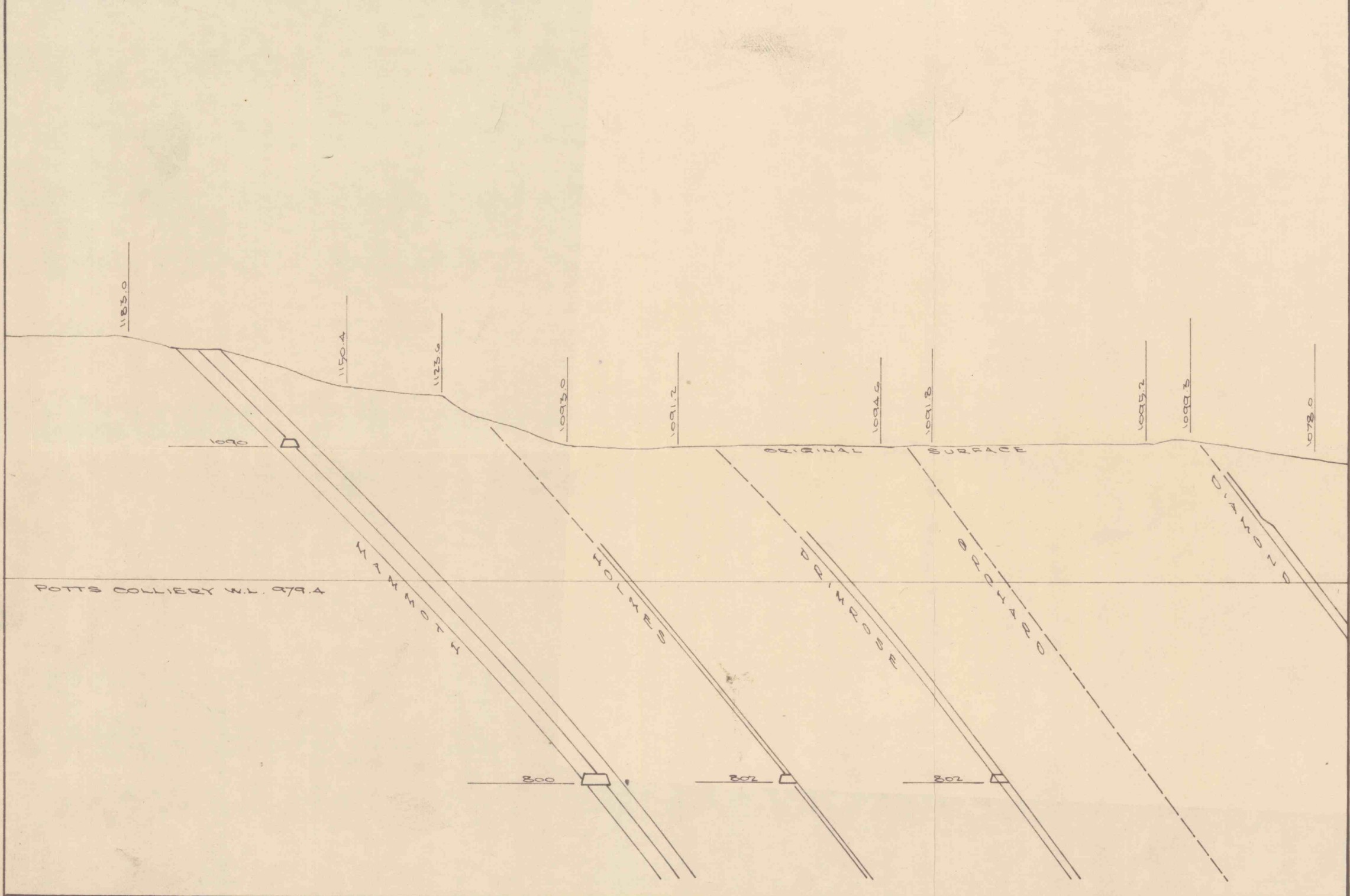
SECTION NO 7 DATUM 700 AMT. - LOOKING EAST SCALE 1"=100'
