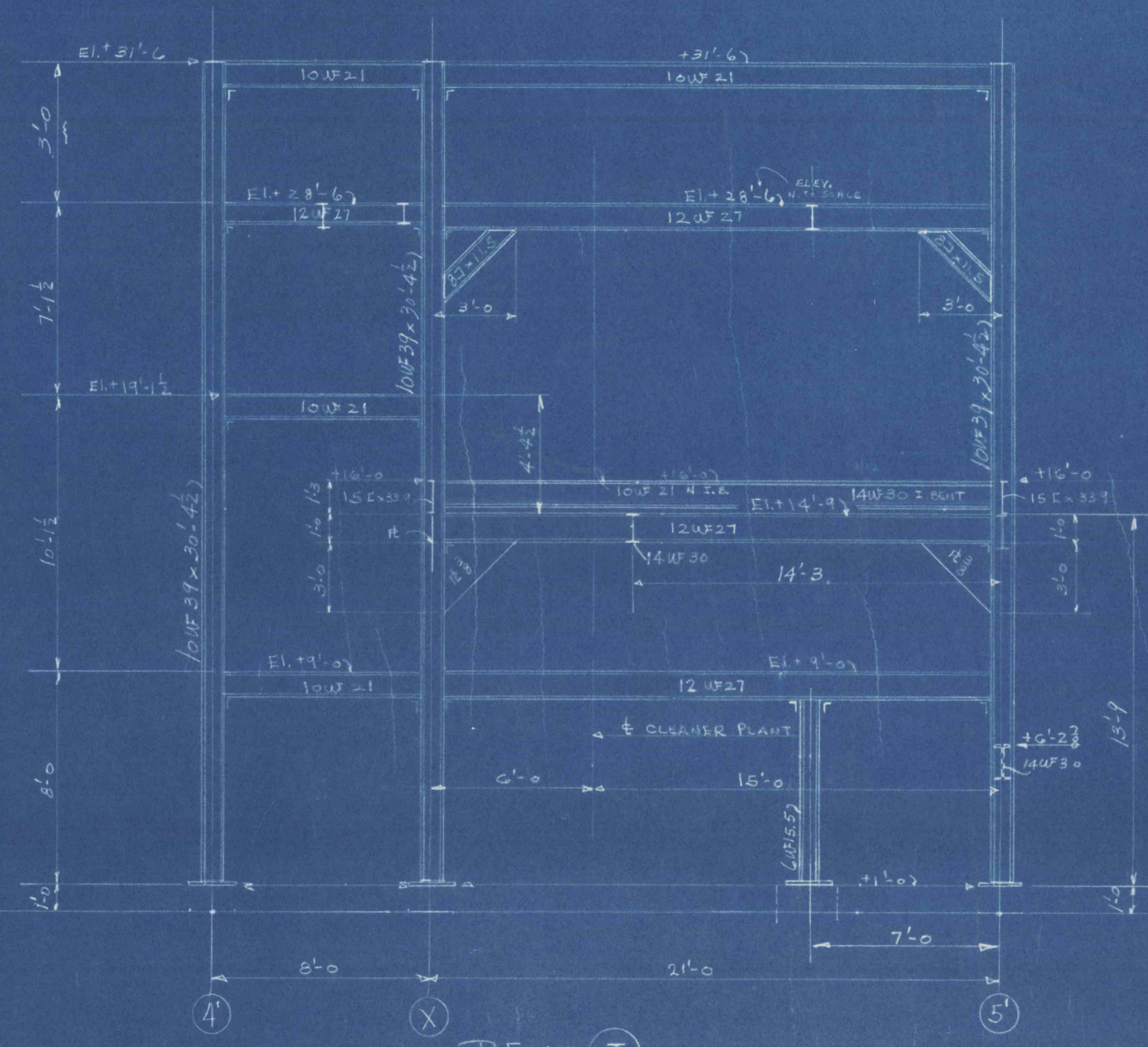
BENT J LOOKING SOUTH
