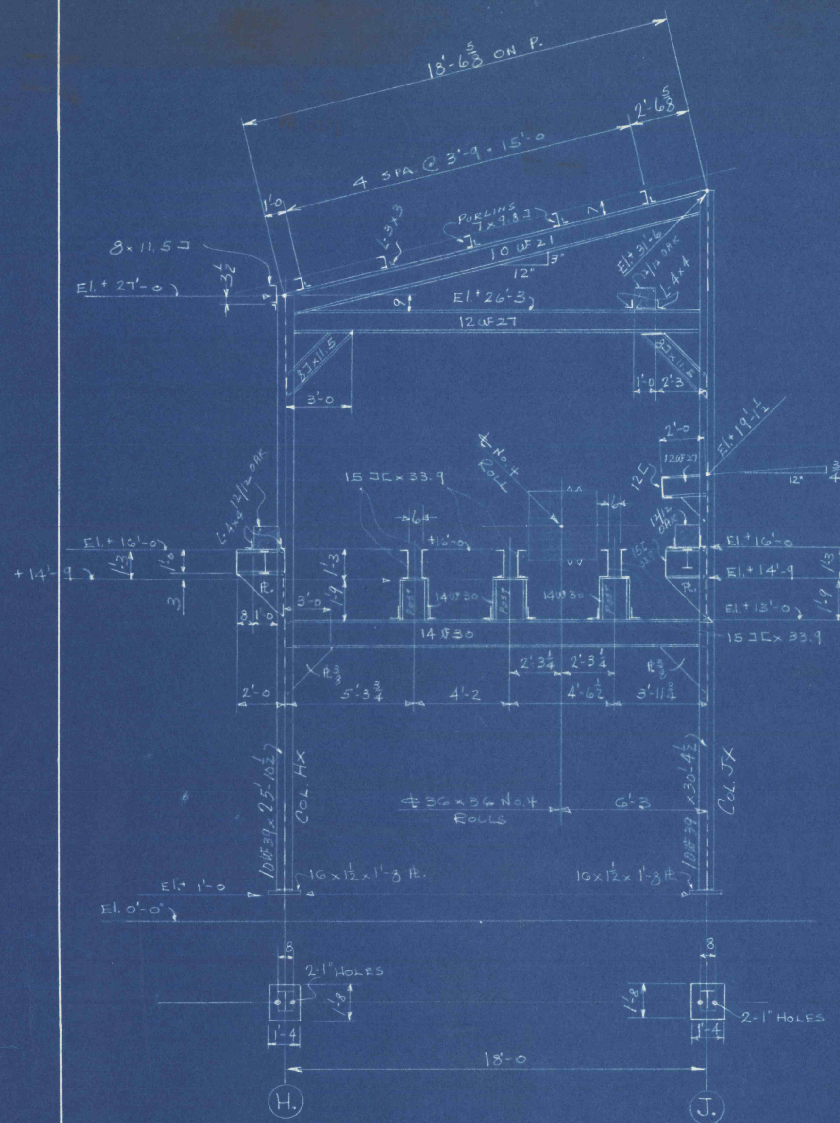
BENT X LOOKING EAST
