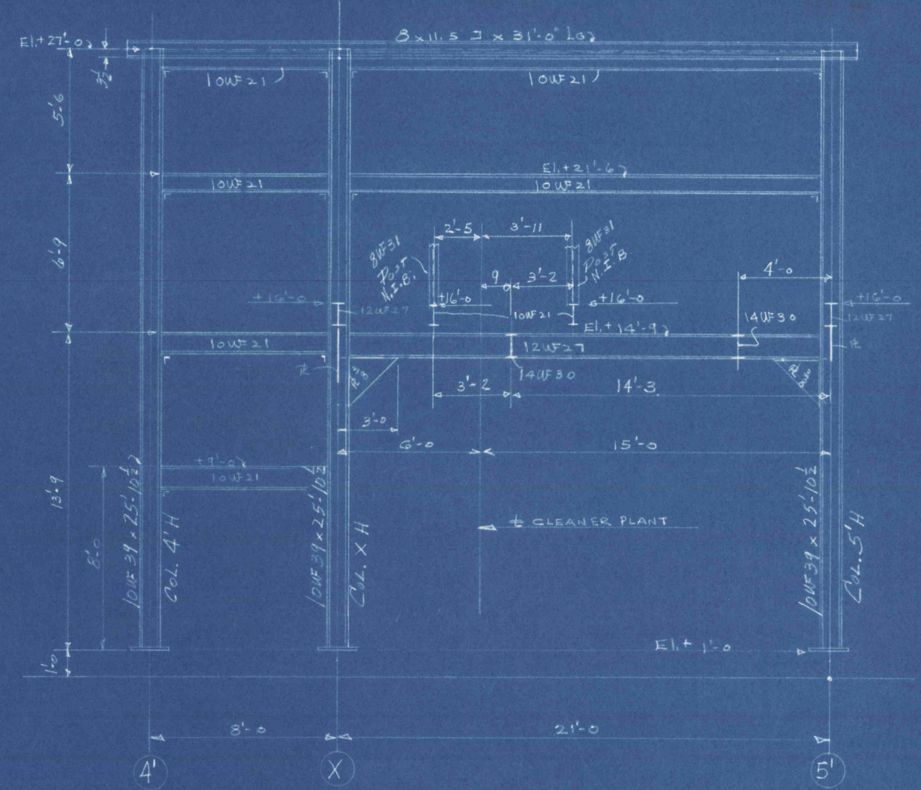
BENT H LOOKING SOUTH
