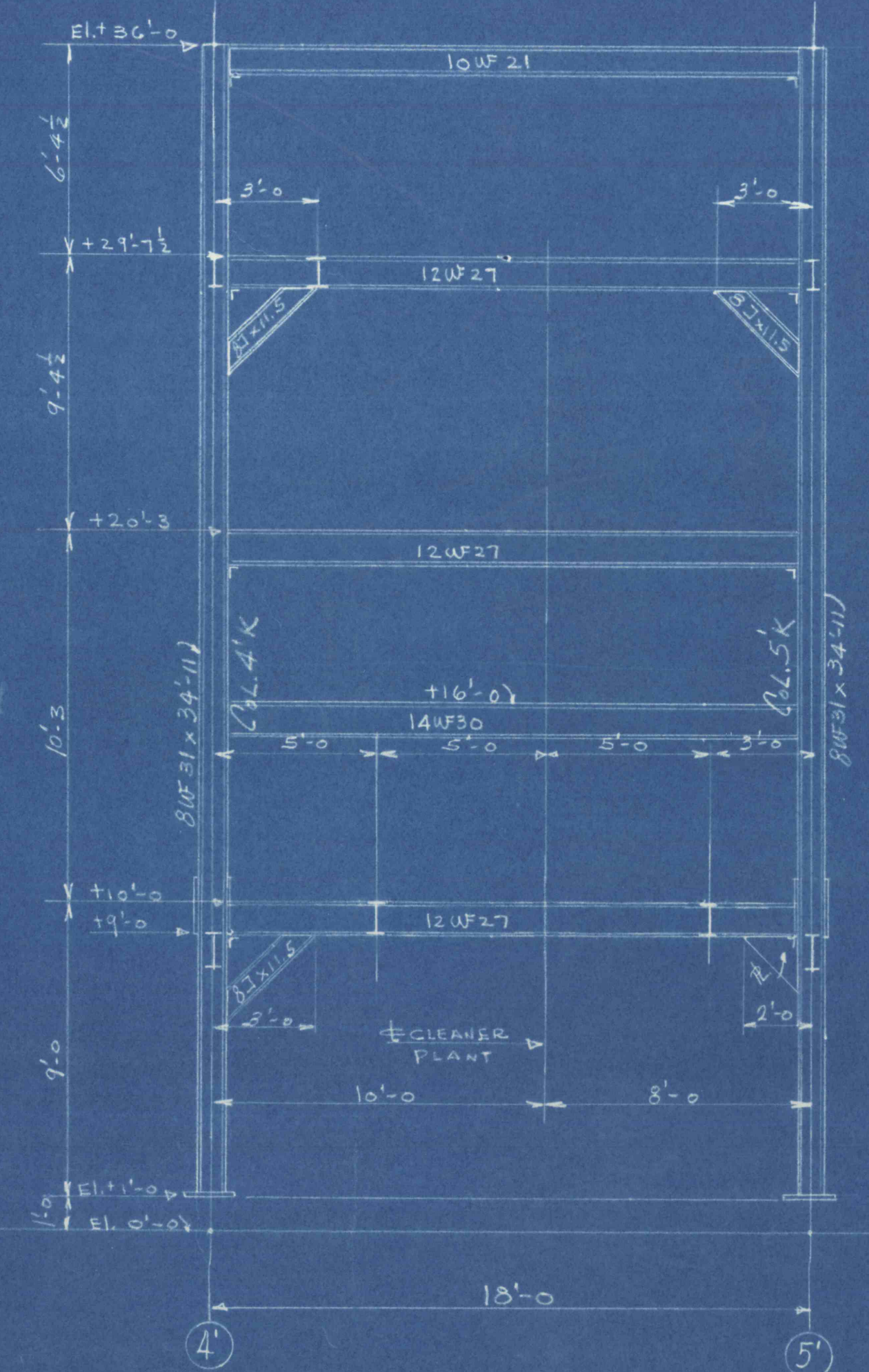
BENT K LOOKING SOUTH
