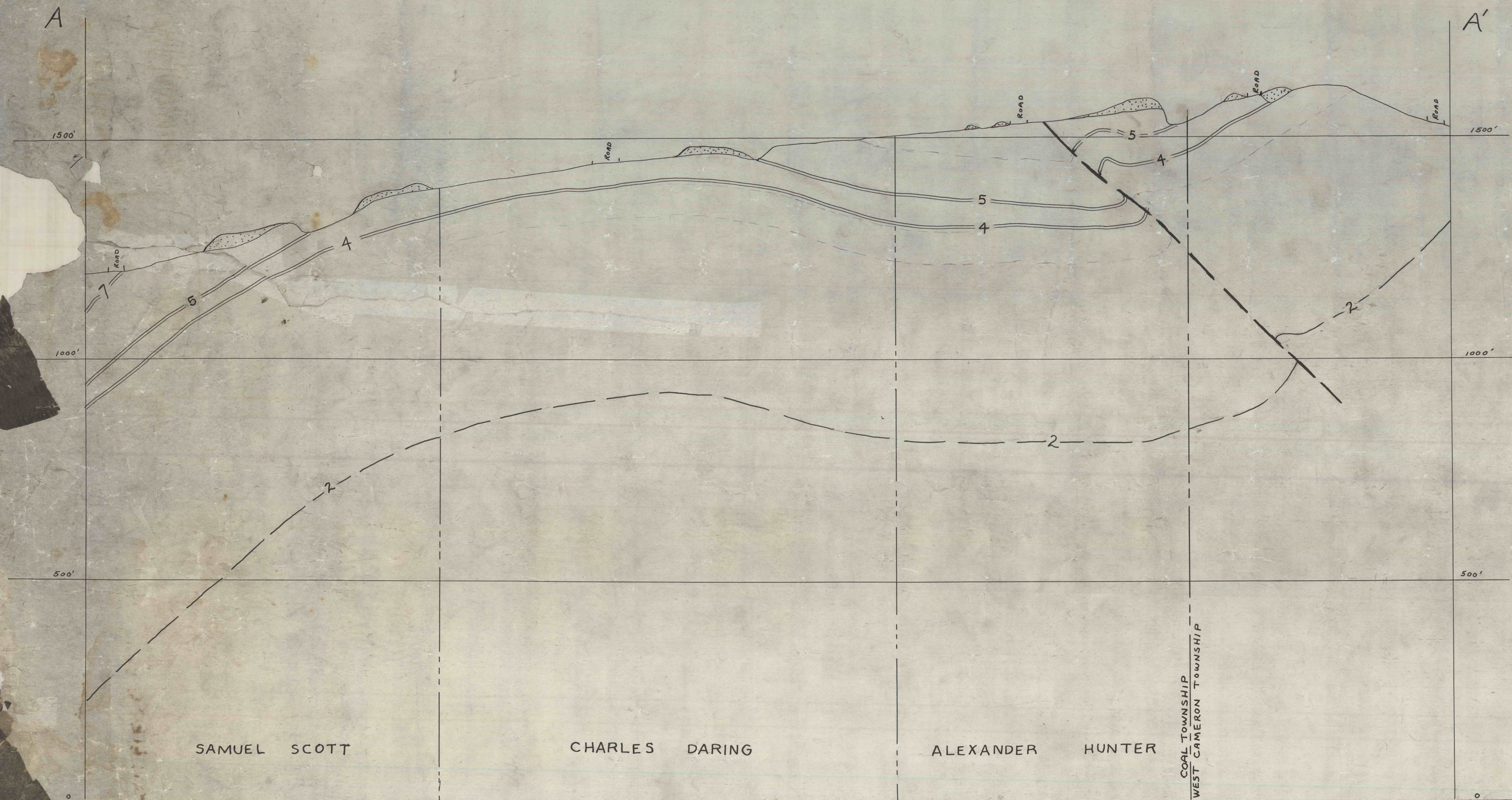
CROSS SECTION A-A' LOOKING EAST SCALE 1" = 100'
