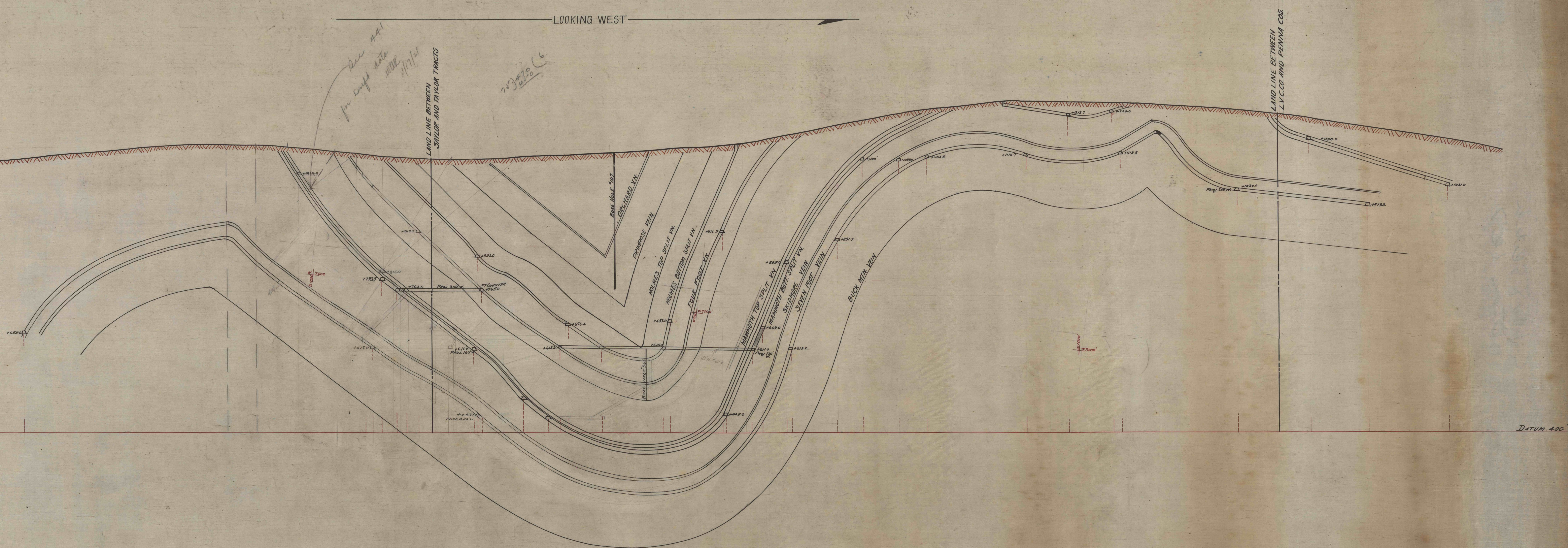
CROSS SECTION THROUGH BARRIER PILLAR BETWEEN SIOUX 1 AND SIOUX 3
