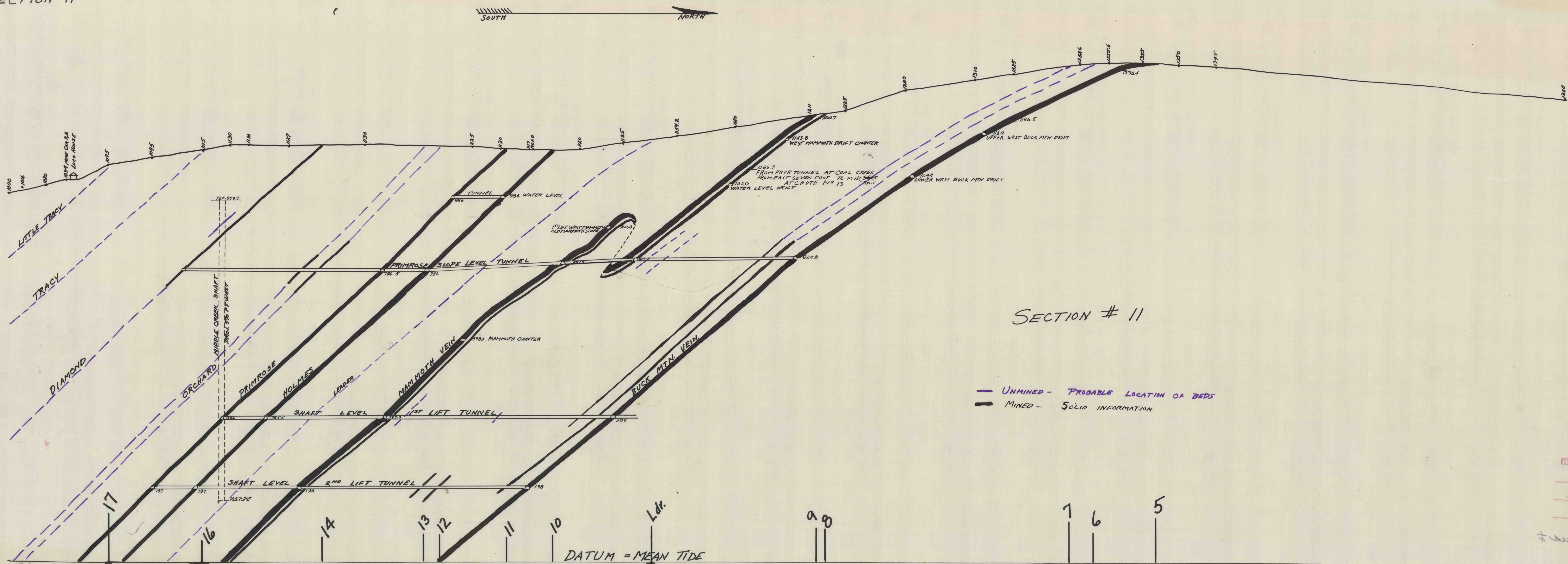
MIDDLE CREEK COLLIERY - CROSS SECTION 570 FEET WEST OF MIDDLE CREEK SHAFT
