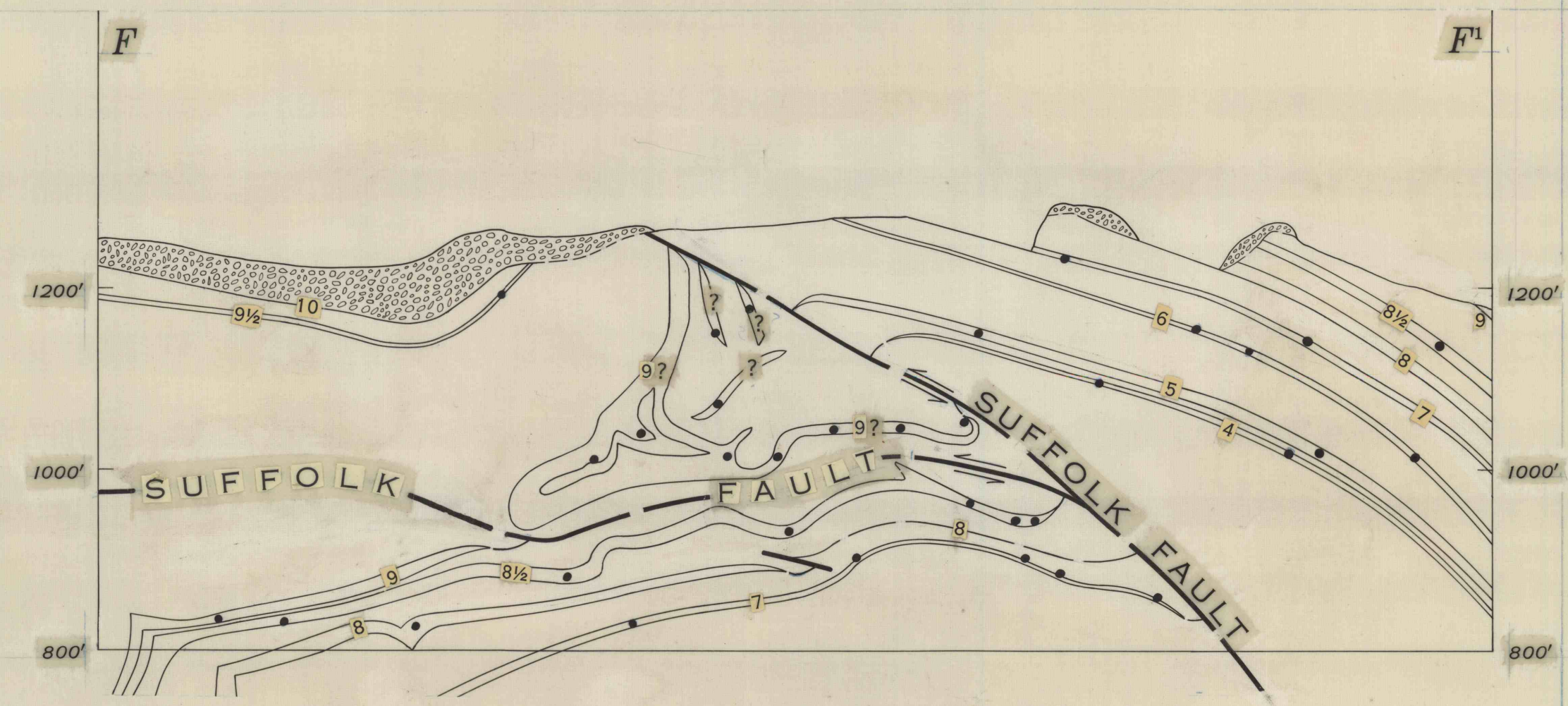
CROSS SECTIONS (LOOKING EAST) SHOWING DEFORMATION OF COAL BEDS ALONG SUFFOLK FAULT
