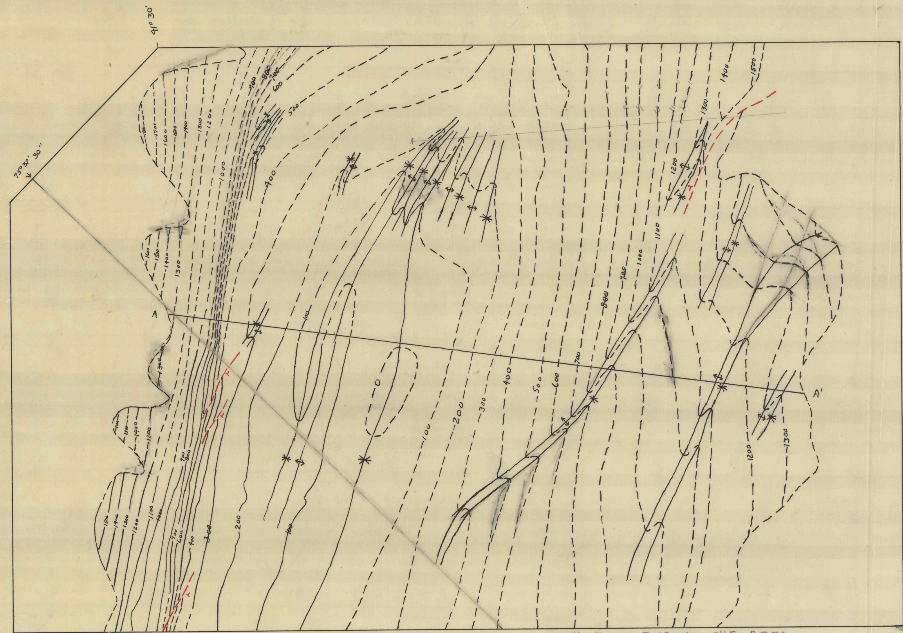
STRUCTURE CONTOUR MAP OF THE LOWER RED ASH COAL BED, IN THE AREA SURROUNDING THE PROPOSED PUMP INSTALLATIONS AT THE JOHNSON COLLIERY
