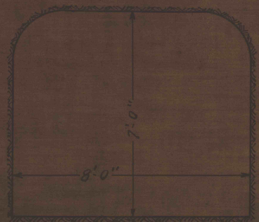
TYPICAL SECTION OF TUNNEL SCALE 1/4" = 1 FT.
