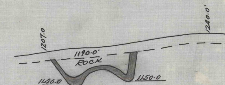
TYPICAL SECTION
