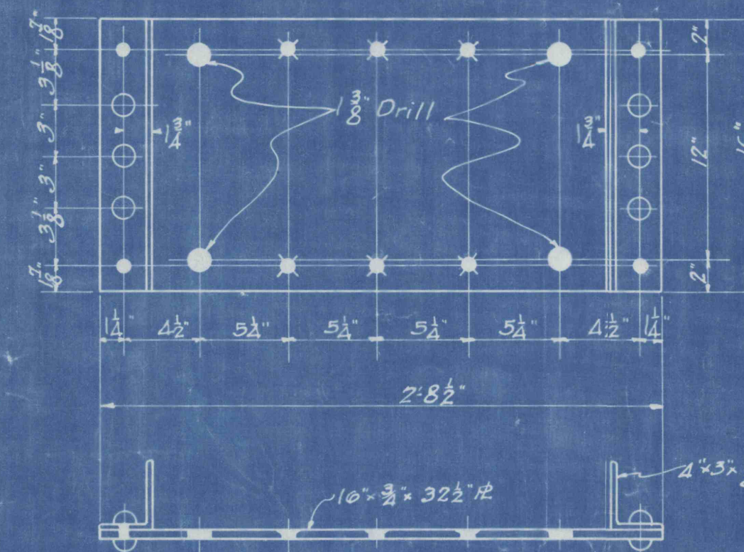
Detail of Base Plate for 4 Front Legs
