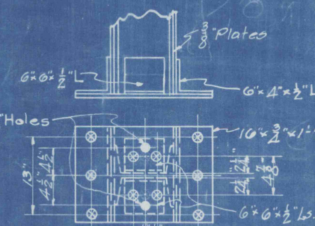
Detail of Base Plate for 4 Front Legs
