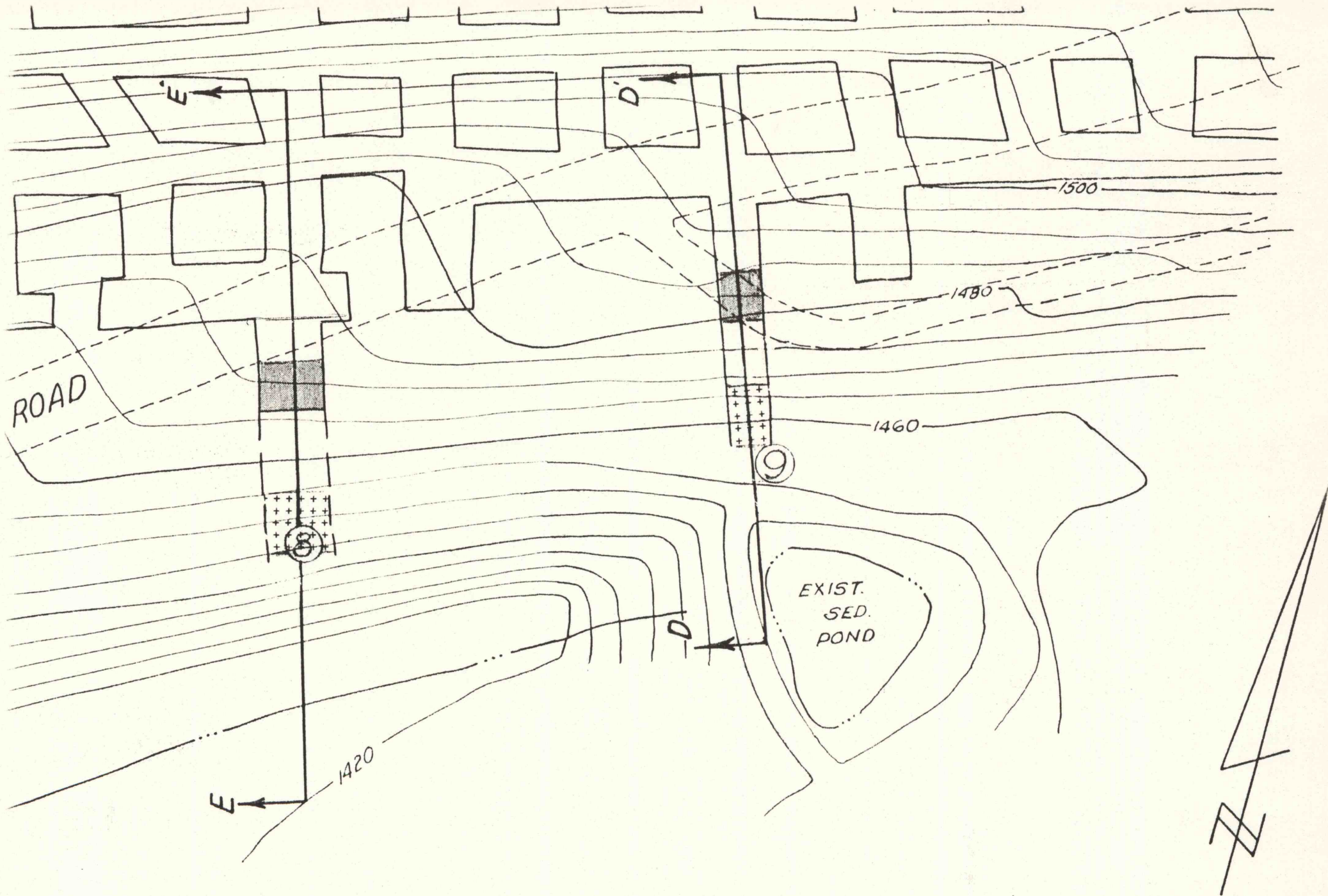
PLAN OF MINE SEALS NO 8 & NO 9 DEEP MINE HYDRAULIC SEALS
