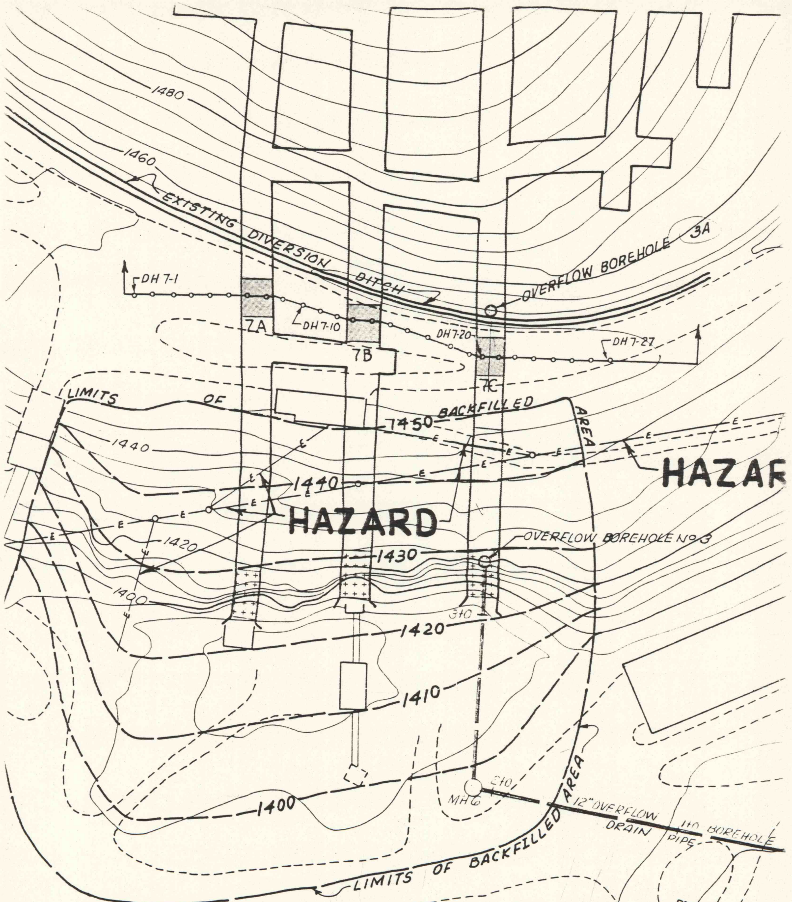
PLAN OF MINE SEAL No 7 DEEP MINE HYDRAULIC SEALS & PRESSURE GROUTING DRILL HOLES
