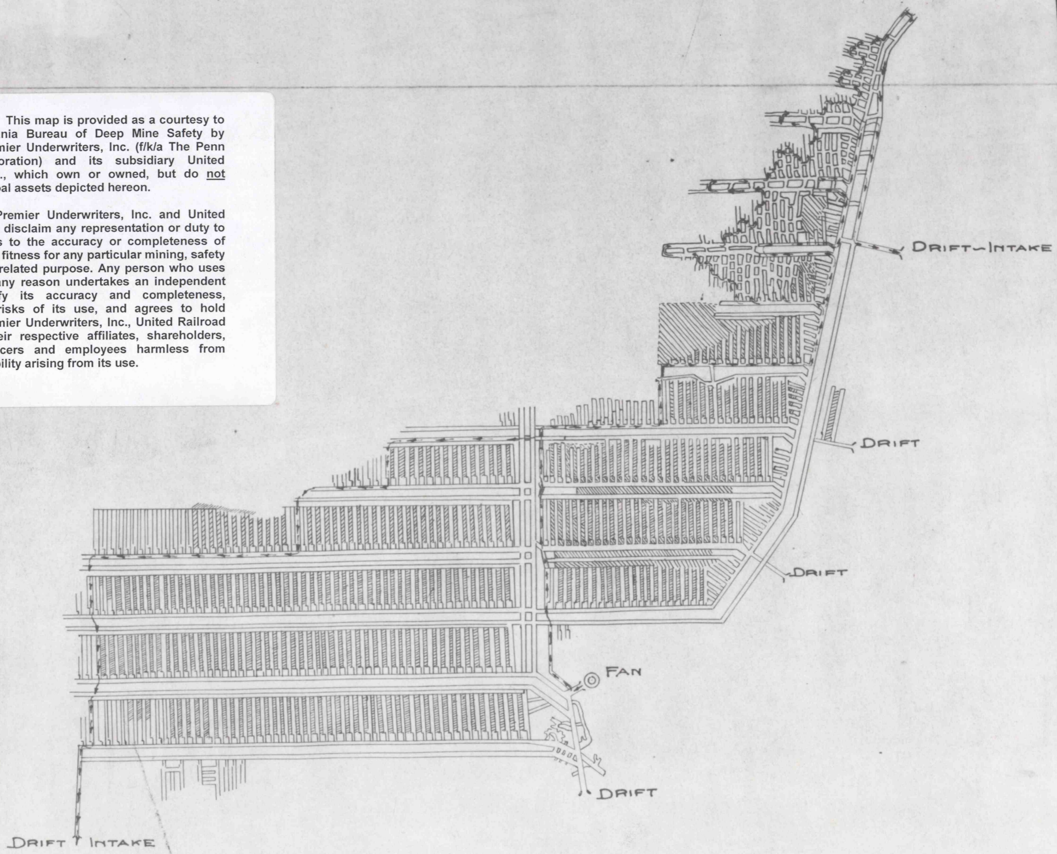
EMPIRE COAL CO. — RODKEY MINE — SCALE 1"=500' ———— DIRECTION OF AIR.
