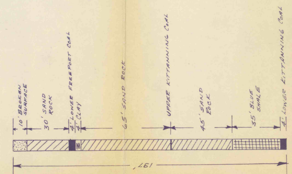
TYPICAL SECTION IN SOME
