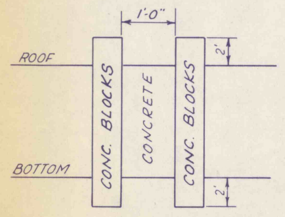
DETAIL OF SEALS
