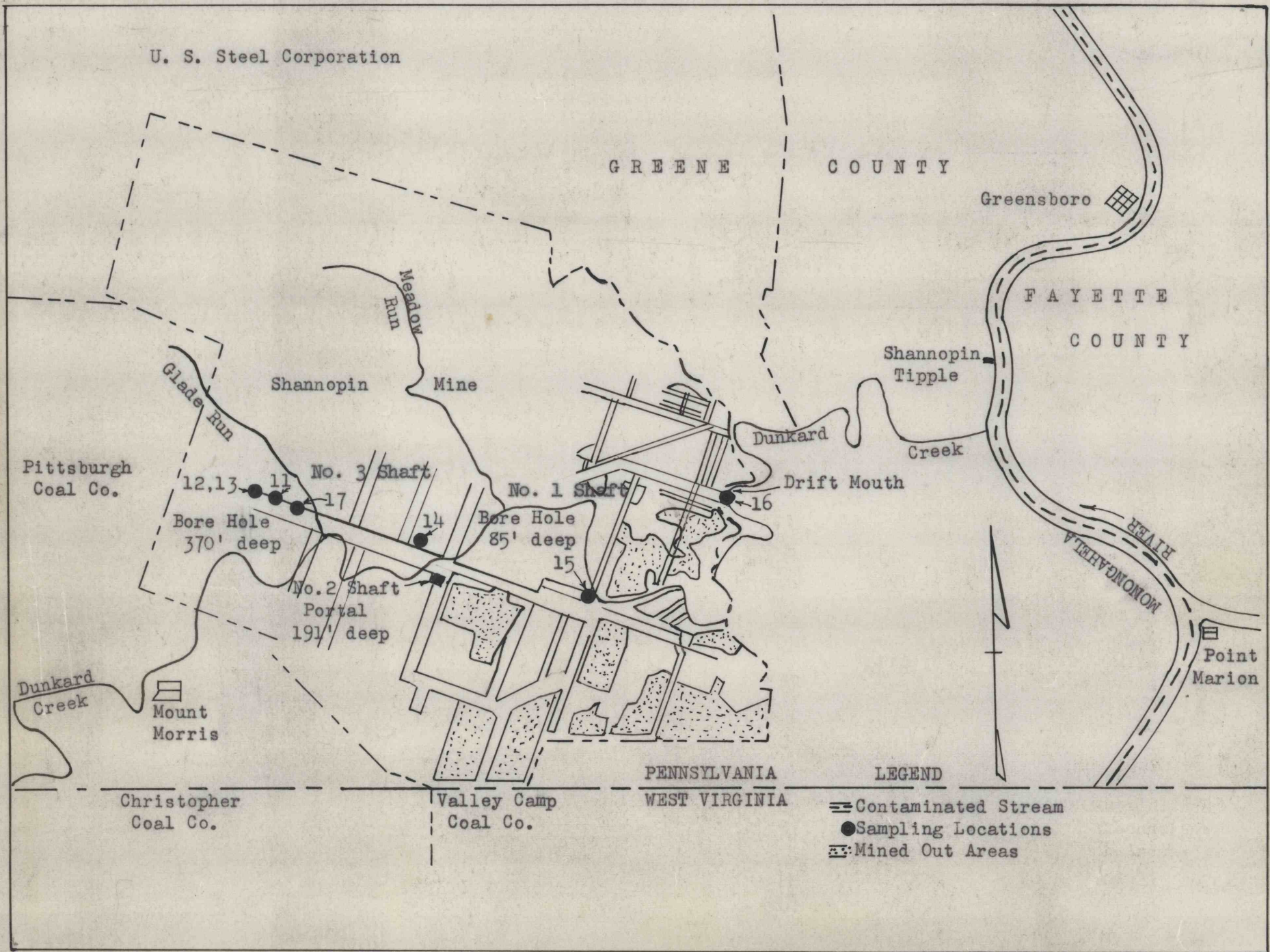
Figure 4. - Sketch map of Pittsburgh bed and surface at the Shannopin mine of Jones and Laughlin Steel Corporation.
