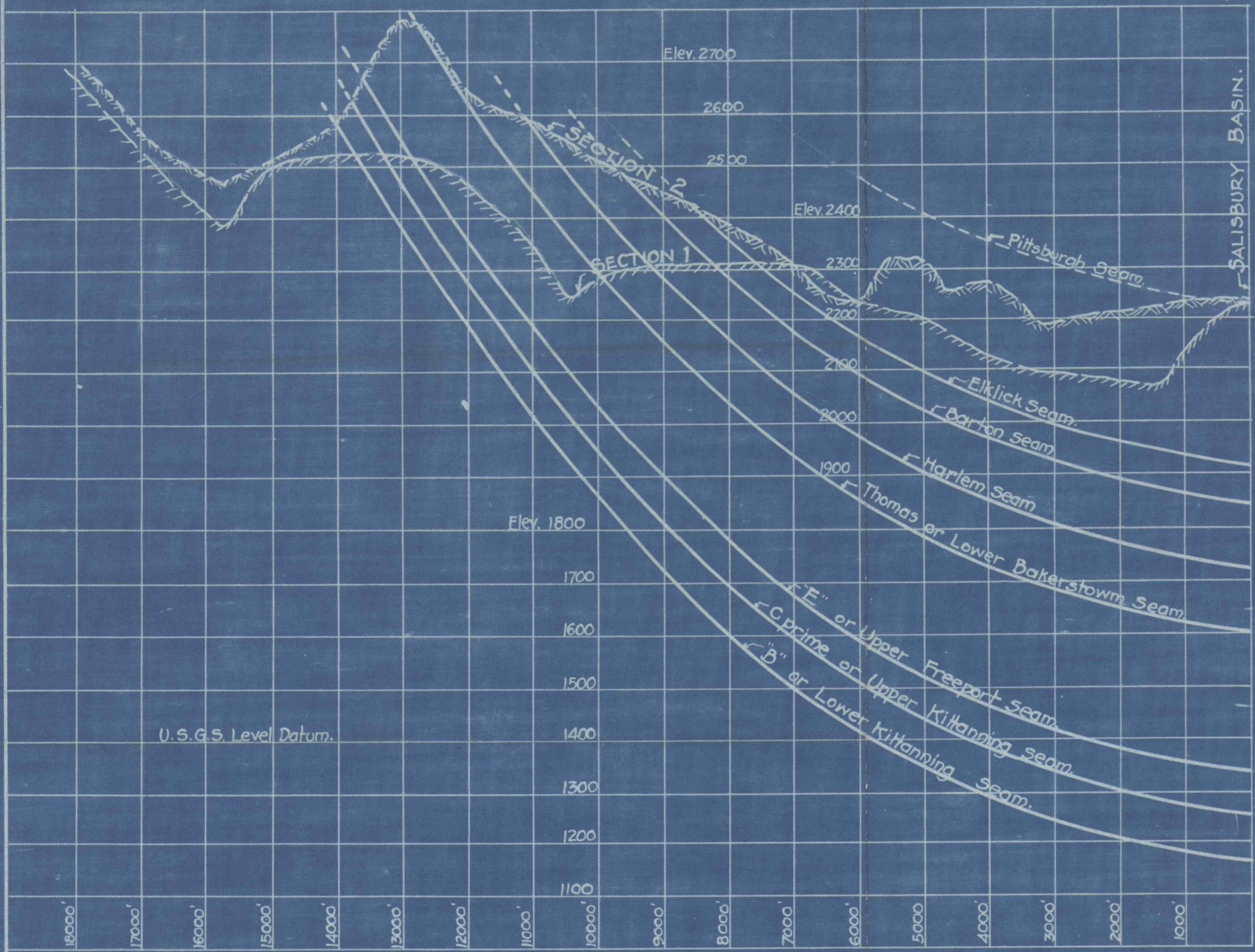
CROSS SECTION SHOWING COAL SEAMS ON WEST SIDE OF SALISBURY BASIN, NEAR TUB MILL MINE. Scale Hor. 1" = 1600' Vert. 1" = 200'
