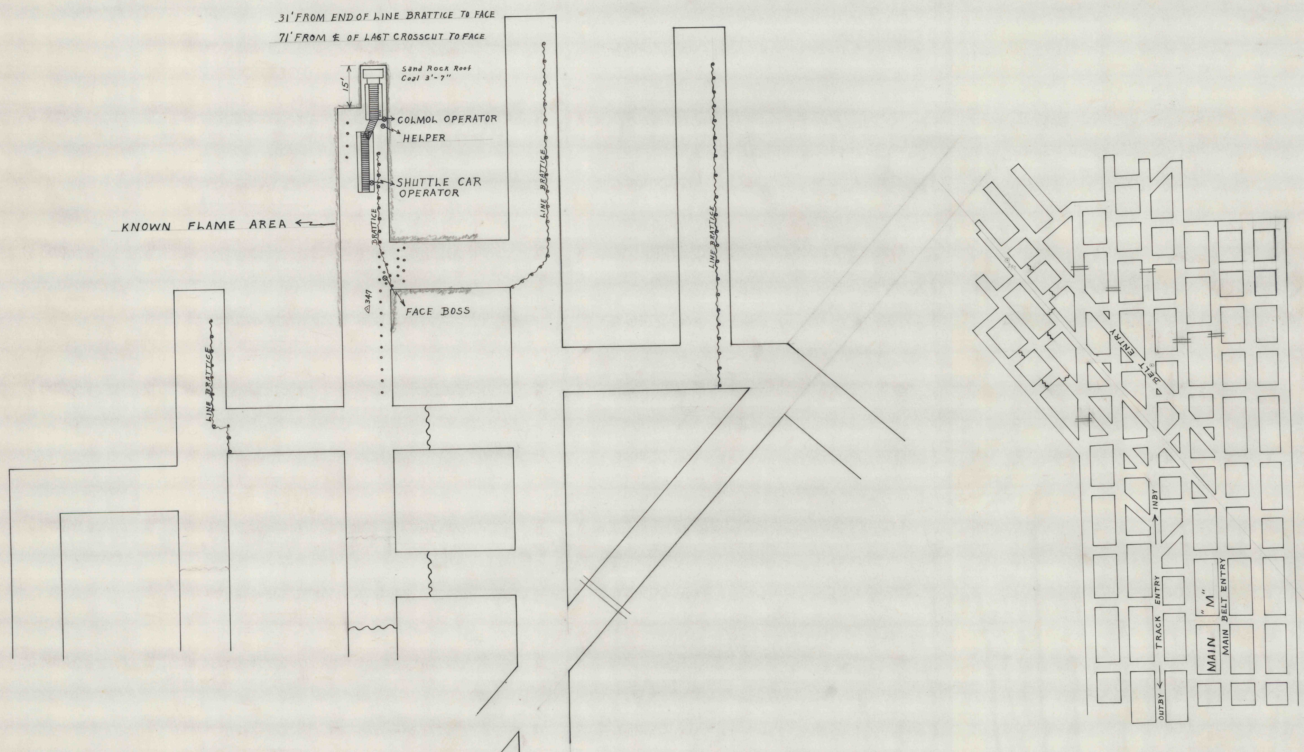
LANCASHIRE No 15 MINE MAIN "M" SECTION IGNITION AREA MAIN ENTRY OCTOBER 26, 1961 SECOND SHIFT SCALE 1"=20'
