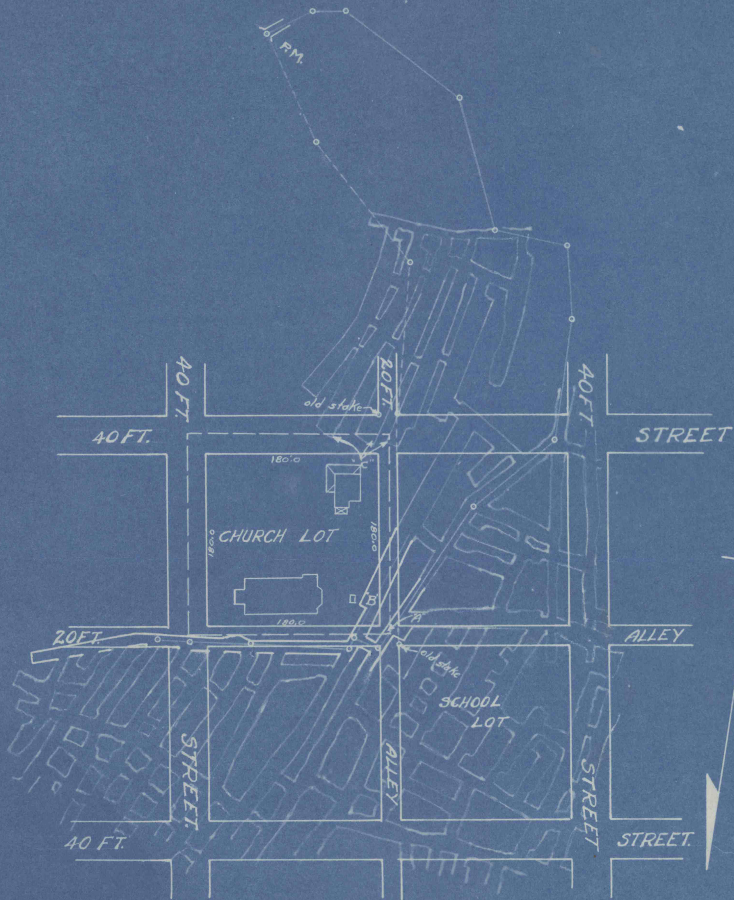
PLOT OF CHECK SURVEY PORTION OF MINE OF THE EDWINA COAL CO. SITUATE IN EAST BETHLEHEM TWP. WASHINGTON CO. PA. SCALE 1 IN. = 100 FT. FEB. 28, 1923.
