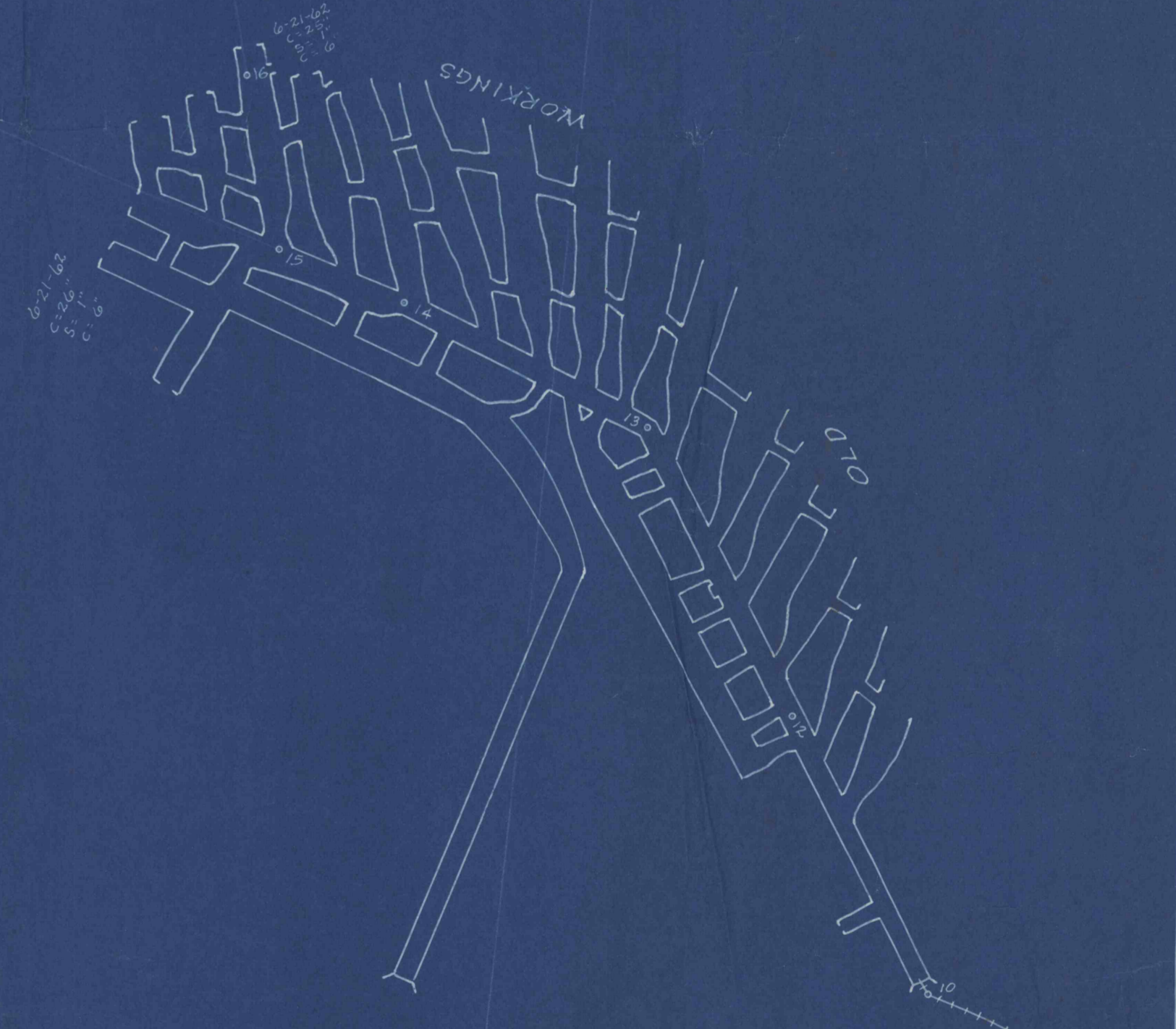
MAP SHOWING "E" SEAM WORKINGS OF BLAIR RICKARD COAL CO. NEAR GLASGOW READE TWP, CAMBRIA CO., PA. SCALE 1"=100' AUG. 20, 1902 J. L. BANFIELD REG. ENG.
