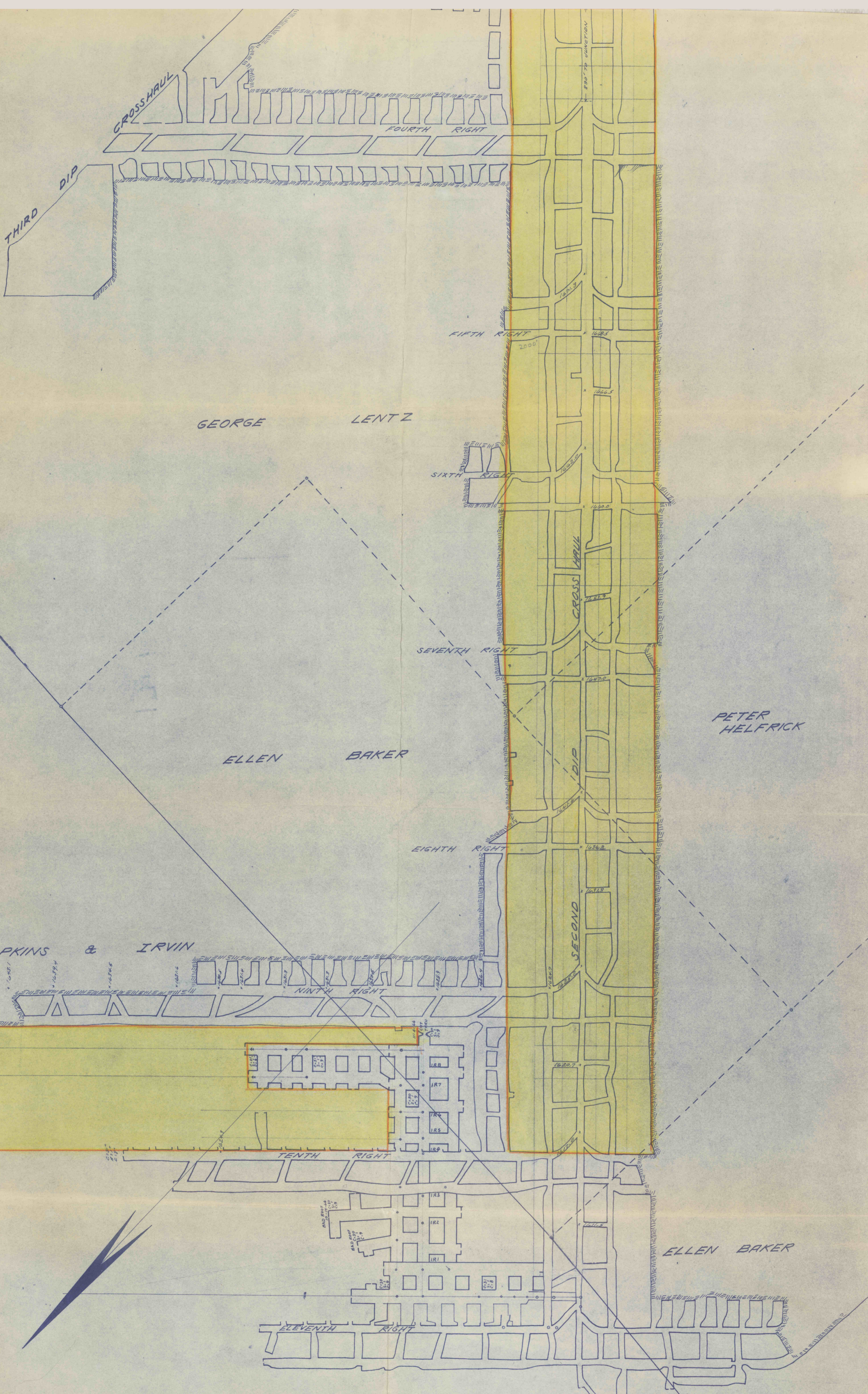
RICH HILL No. 1 MINE PROJECTED WORKING AREAS - "E" SEAM DECEMBER 1, 1966 TO JUNE 1, 1967 1" = 100'
