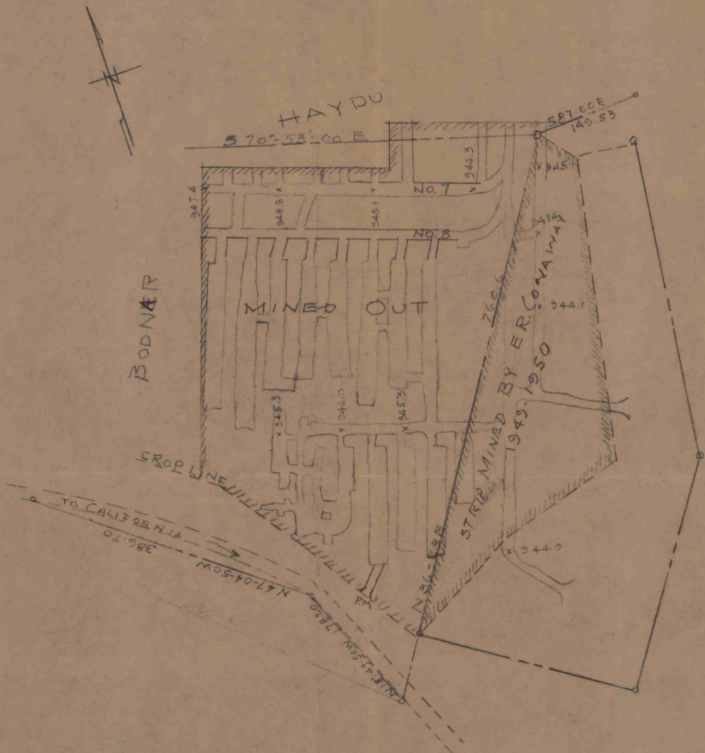
PORTION OF CRESCENT NO. 1 MINE MINED BY MIKE BODNAR AND STEPHEN H. BODNAR WEST PIKE RUN TWP. WASHINGTON CO. PA SCALE 1"=100' 3-24-62
