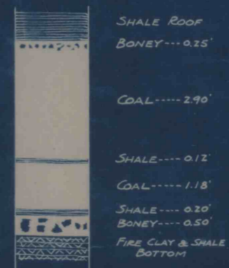
TYPICAL SECTION OF COAL SEAM
