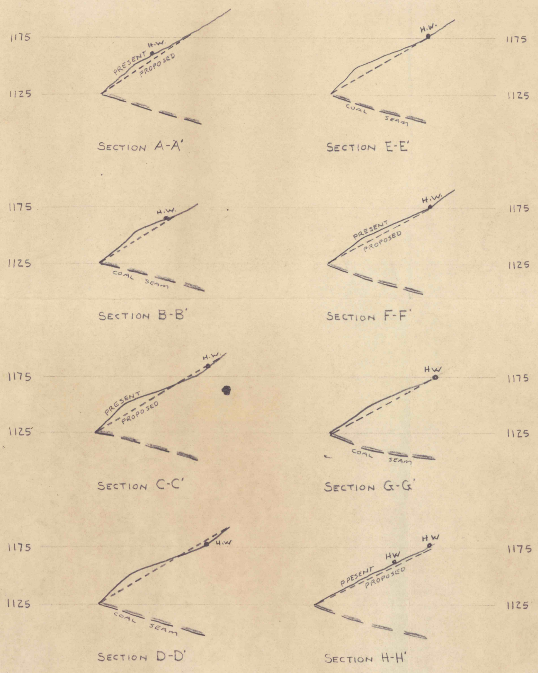
CROSS SECTIONS SCALE HORZ 1"=200' VERT. 1"=50'
