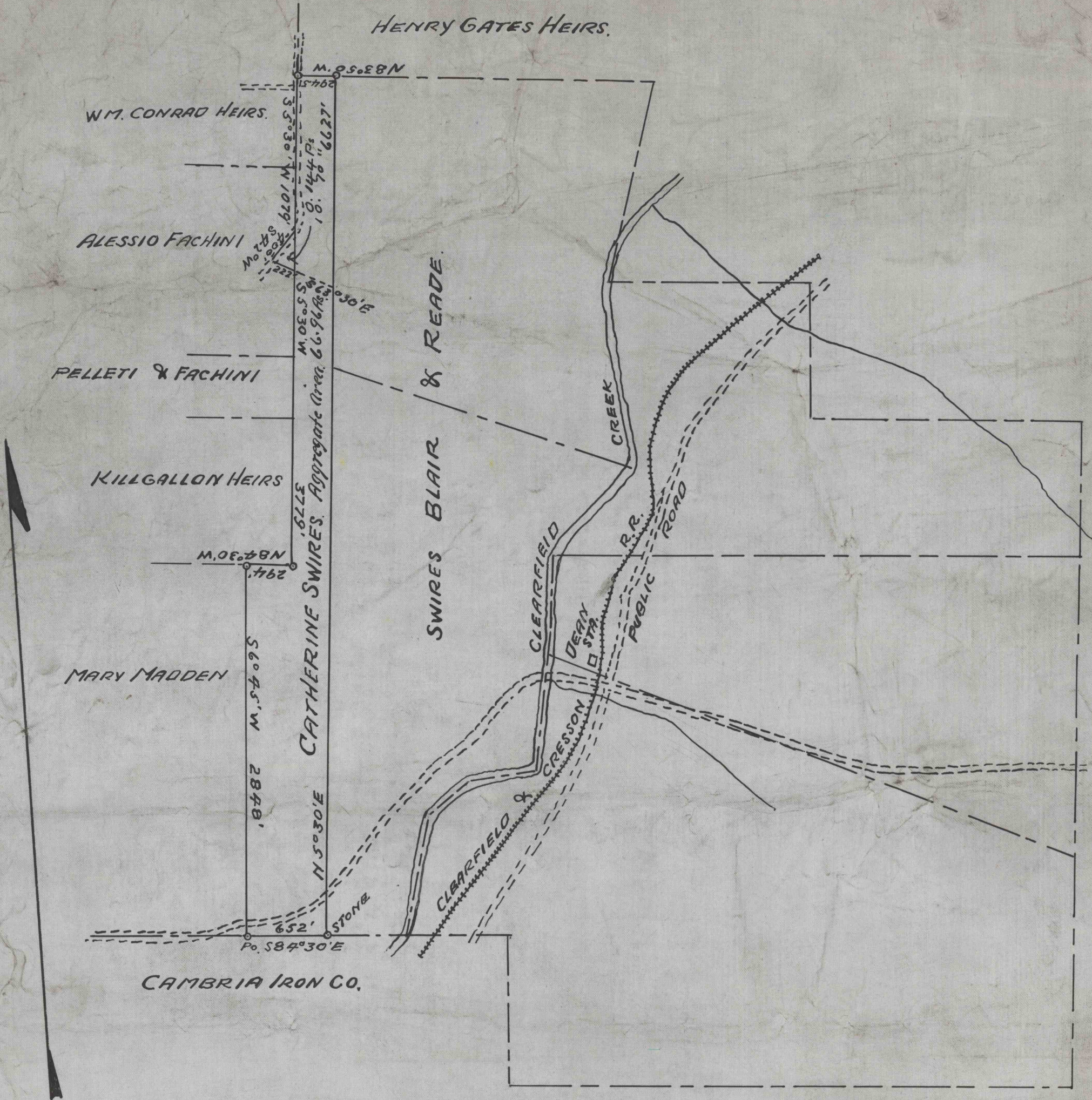
Situate on the Waters of Clearfield Creek Dean Township Cambria County, Penna., Surveyed for John Tierney, April 1925, Scale 1" = 800' P.F. Campbell Engr.
