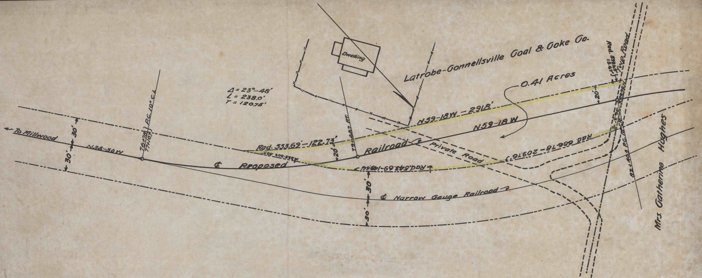
BARNETT COAL CO MAP SHOWING LAND TO BE ACQUIRED FOR SIDING TO OLD MILLWOOD SHAFT THROUGH LATROBE-GONNELLSVILLE COAL & COKE CO. Scale - 1" = 50' Albert Smith, C. E., 28 Blairsville, Pa. 9/30/20
