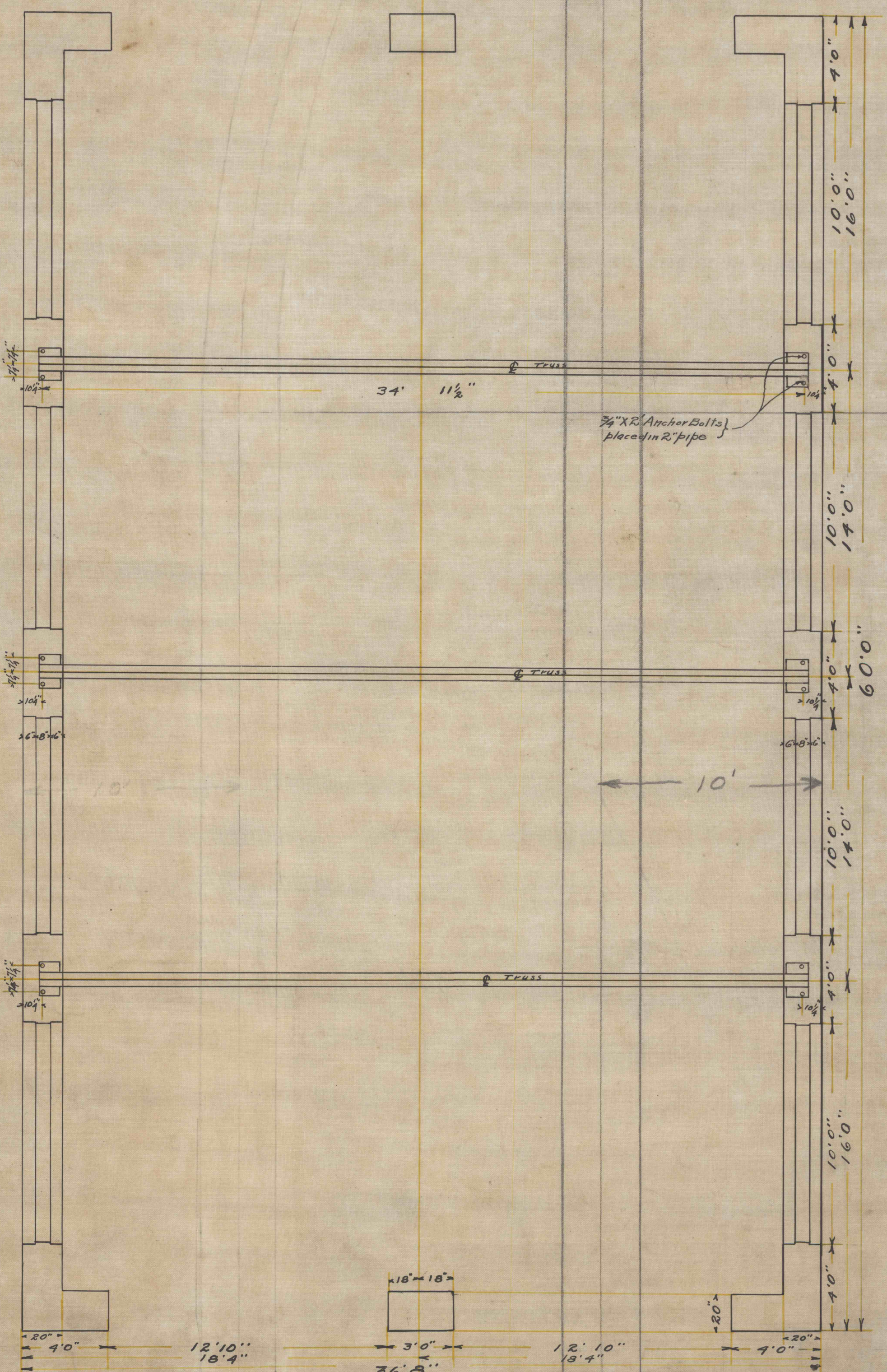
FOUNDATION PLAN
