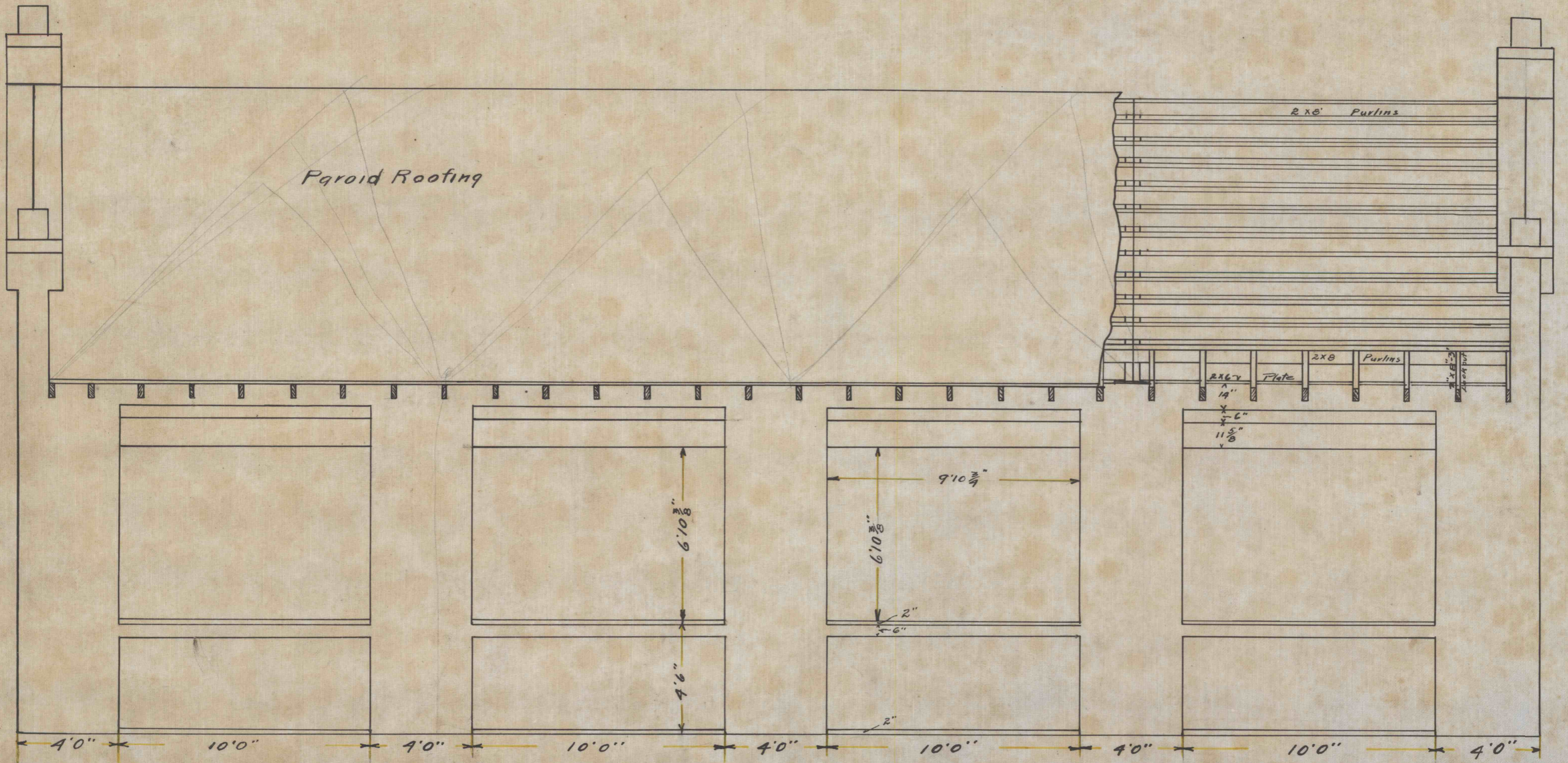
SIDE ELEVATION
