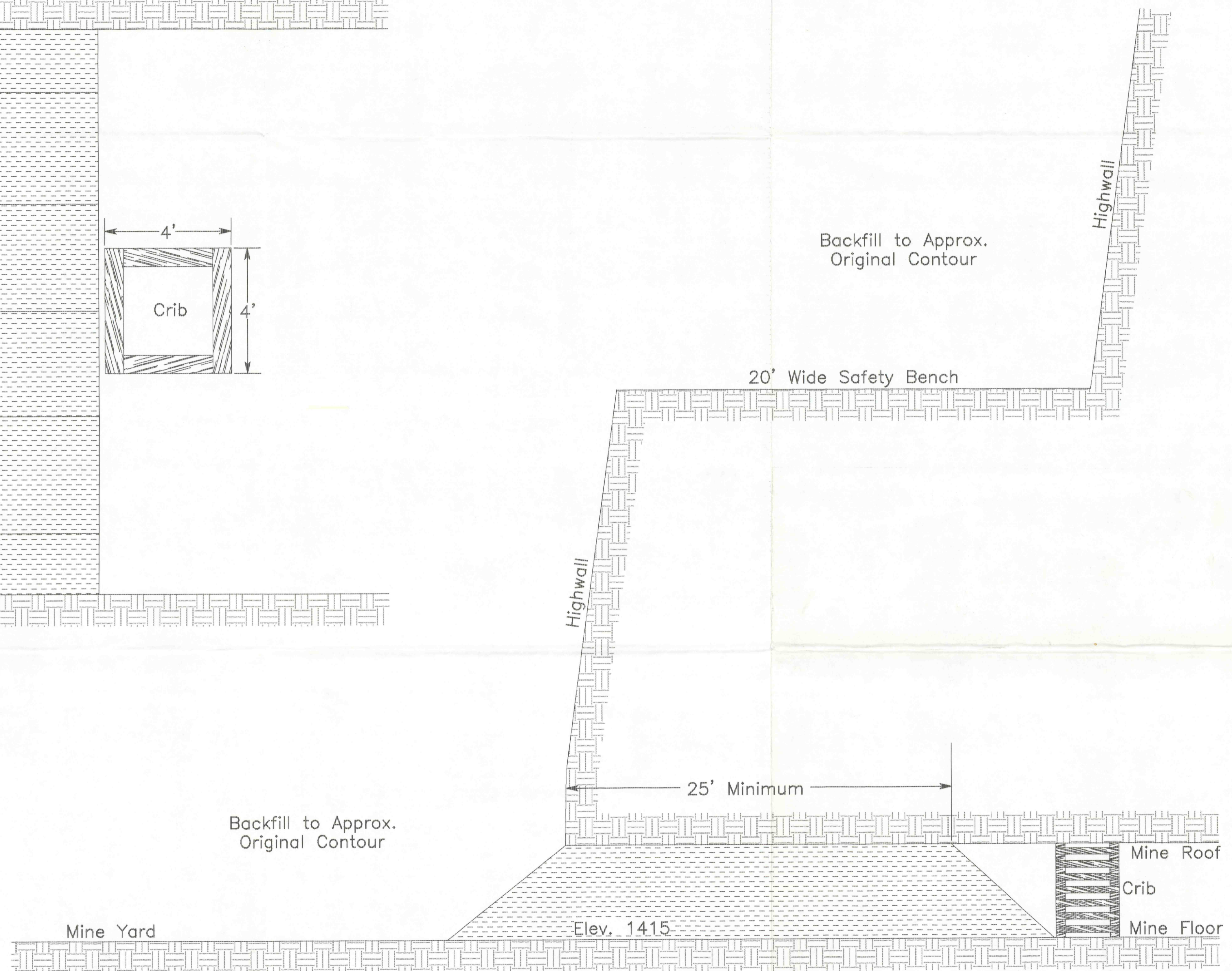
Mine Seal — Side View
