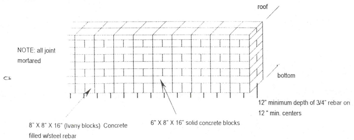
Typical Construction Detail
