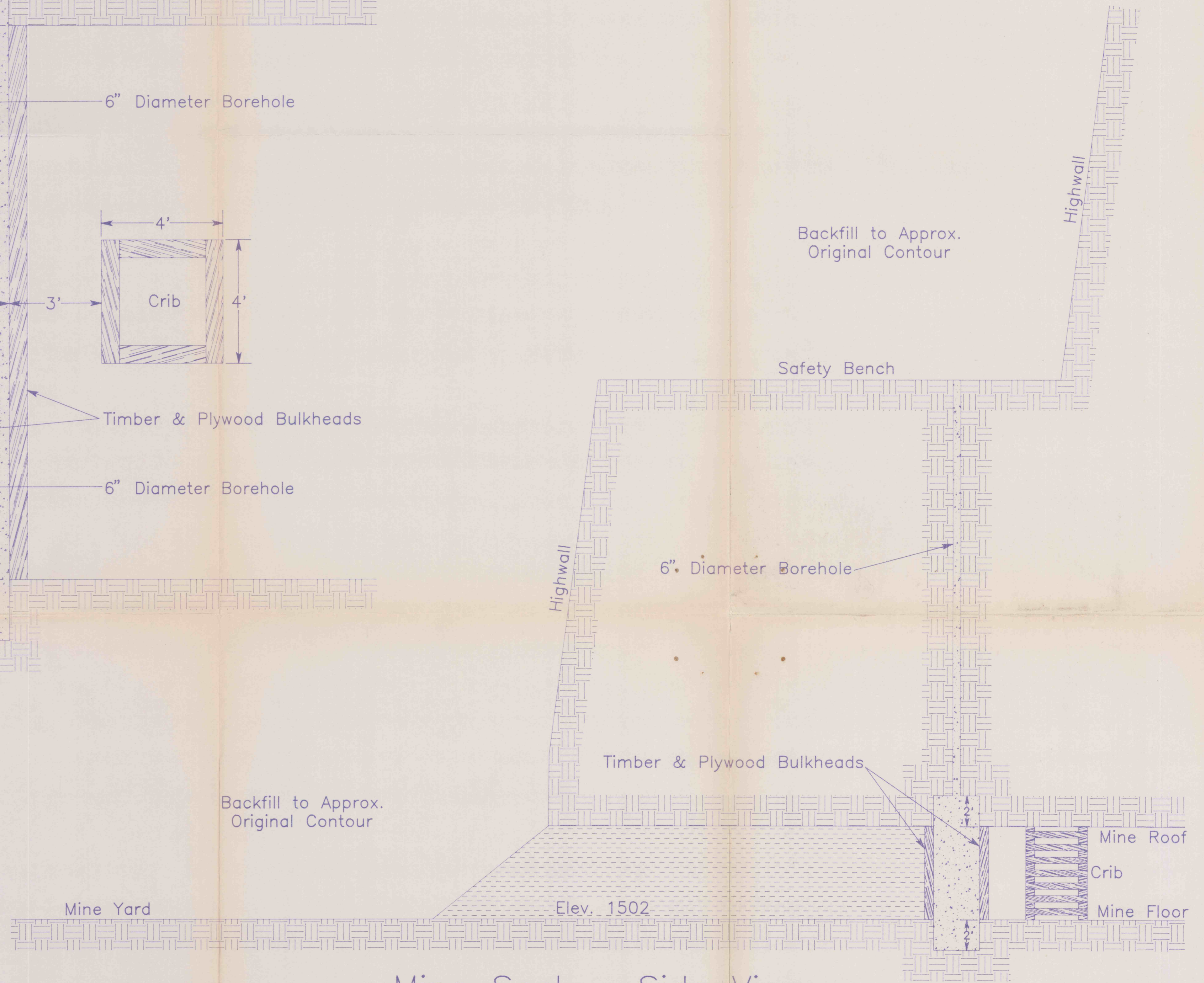
Mine Seal — Side View
